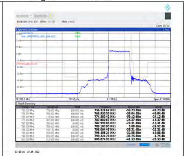
1-N14--15-10-L-3-DFT-PI2BPSK-Outer_Full-50@0-Ant1-PASS-see graph
