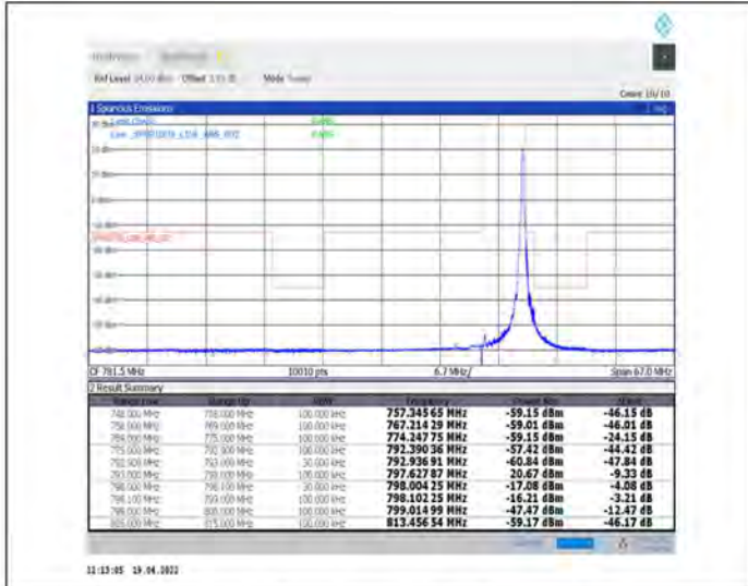
1-N14--15-5-H-2-DFT-PI2BPSK-Edge_1RB_Right-1@24-Ant1-PASS-see graph
