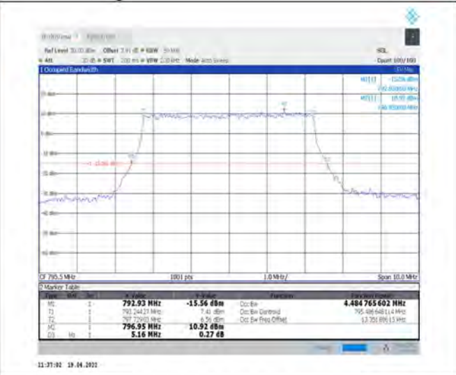
1-N14--15-5-H-8-CP-64QAM-Outer_Full-25@0-Ant1-4.485-5.160-≤5-PASS
