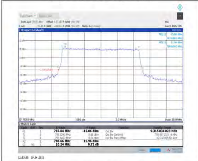
1-N14--15-10-H-6-CP-QPSK-Outer_Full-52@0-Ant1-9.316-10.240-≤10-PASS
