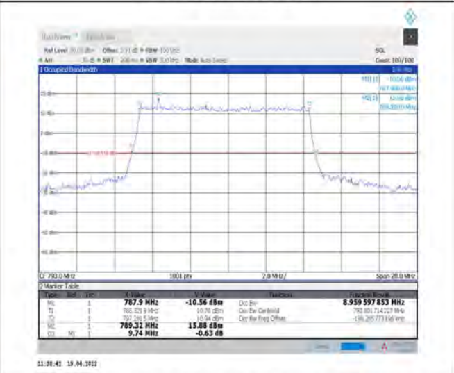
1-N14--15-10-L-1-DFT-QPSK-Outer_Full-50@0-Ant1-8.96-9.740-≤10-PASS
