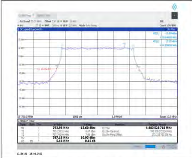
1-N14--15-5-H-7-CP-16QAM-Outer_Full-25@0-Ant1-4.484-5.160-≤5-PASS
