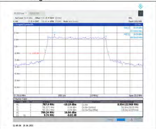
1-N14--15-10-H-1-DFT-QPSK-Outer_Full-50@0-Ant1-8.954-9.740-≤10-PASS
