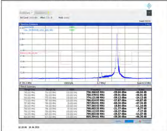
1-N14--15-10-H-5-CP-QPSK-Edge_1RB_Right-1@51-Ant1-PASS-see graph
