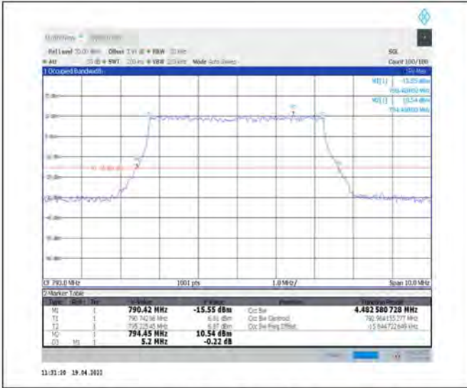
1-N14--15-5-M-8-CP-64QAM-Outer_Full-25@0-Ant1-4.483-5.200-≤5-PASS
