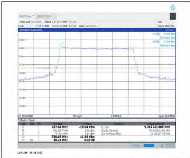
1-N14--15-10-L-6-CP-QPSK-Outer_Full-52@0-Ant1-9.314-10.240-≤10-PASS
