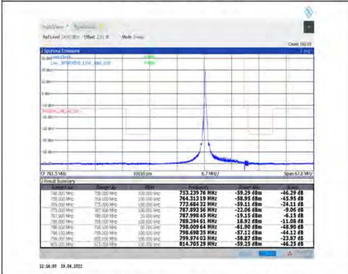
1-N14--15-10-L-4-CP-QPSK-Edge_1RB_Left-1@0-Ant1-PASS-see graph
