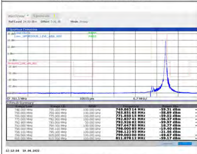
1-N14--15-5-H-5-CP-QPSK-Edge_1RB_Right-1@24-Ant1-PASS-see graph
