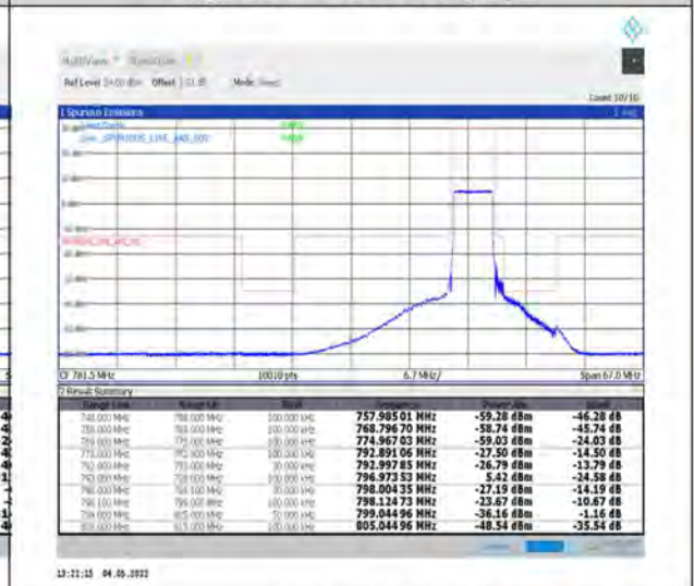
1-N14--15-5-H-6-CP-QPSK-Outer_Full-25@0-Ant1-PASS-see graph
