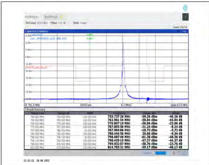
1-N14--15-10-L-1-DFT-PI2BPSK-Edge_1RB_Left-1@0-Ant1-PASS-see graph
