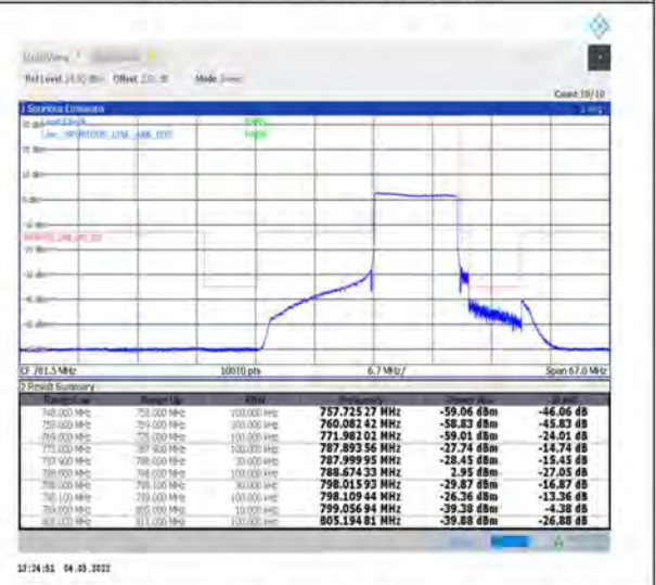
1-N14--15-10-H-6-CP-QPSK-Outer_Full-52@0-Ant1-PASS-see graph
