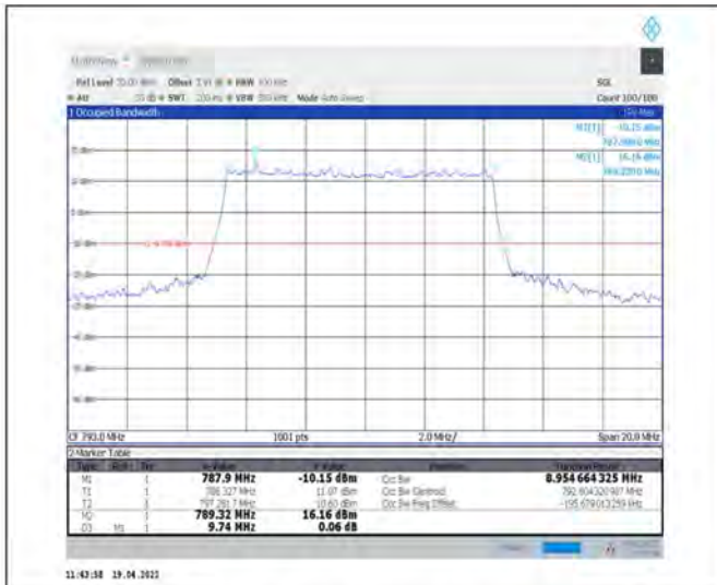
1-N14--15-10-M-1-DFT-QPSK-Outer_Full-50@0-Ant1-8.955-9.740-≤10-PASS
