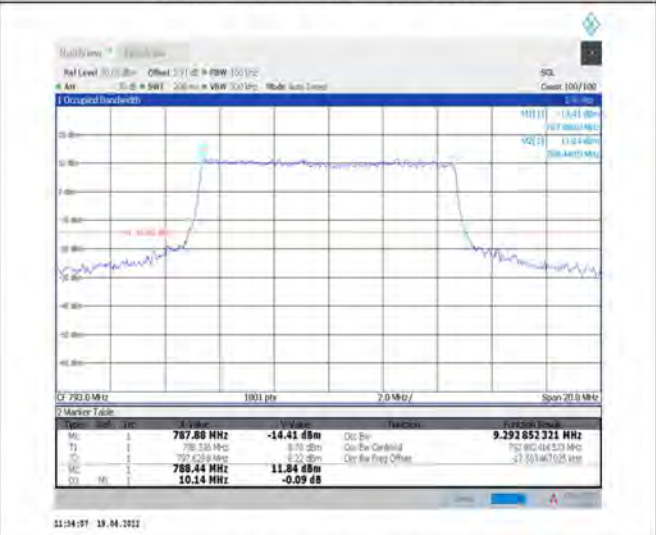
1-N14--15-10-H-7-CP-16QAM-Outer_Full-52@0-Ant1-9.293-10.140-≤10-PASS
