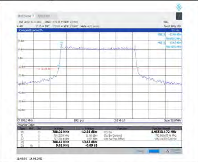
1-N14--15-10-L-3-DFT-16QAM-Outer_Full-50@0-Ant1-8.956-9.620-≤10-PASS
