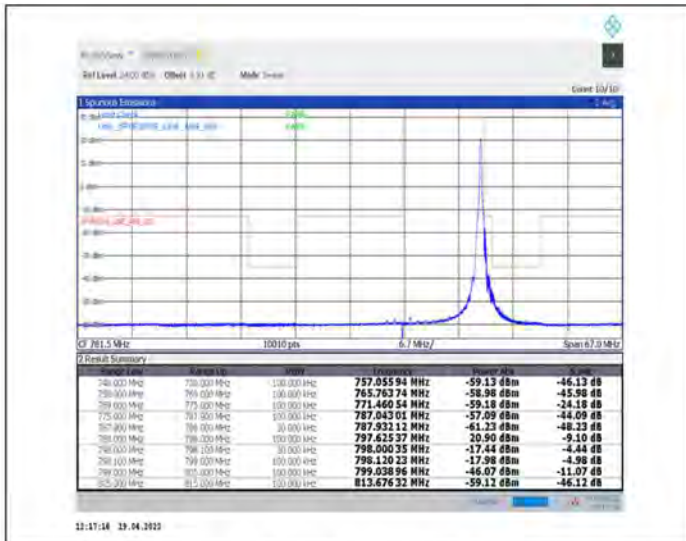
1-N14--15-10-H-2-DFT-PI2BPSK-Edge_1RB_Right-1@51-Ant1-PASS-see graph
