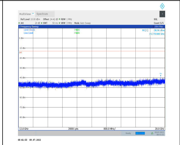
1-N13--15-10-M-1-DFT-PI2BPSK-Inner_1RB_Left-1 @1-12000-20000-Ant1--38.96--13-PASS
