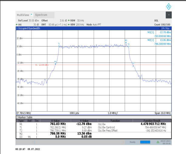
1-N13--15-5-H-2-DFT-PI2BPSK-Outer_Full-25@0-Ant1- 4.479-5.000-≤5-PASS
