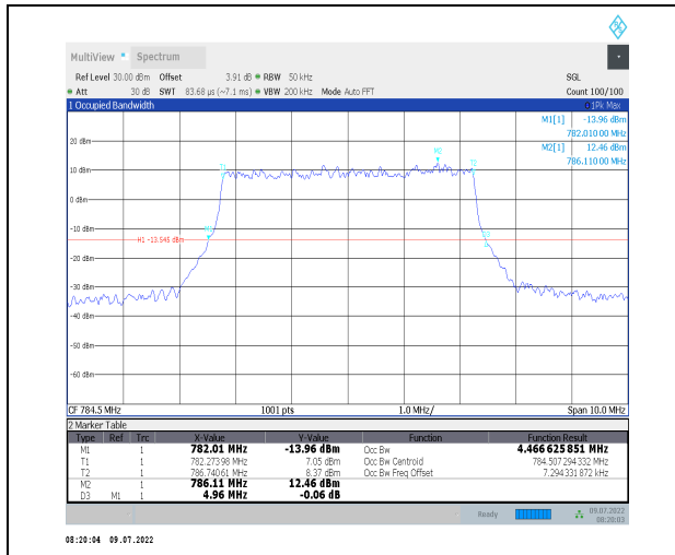
1-N13--15-5-H-3-DFT-16QAM-Outer_Full-25@0-Ant 1-4.467-4.960- \leq 5 -PASS
