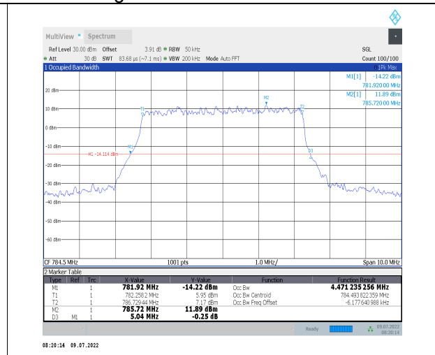
1-N13--15-5-H-4-DFT-64QAM-Outer_Full-25@0-Ant 1-4.471-5.040- \leq 5 -PASS
