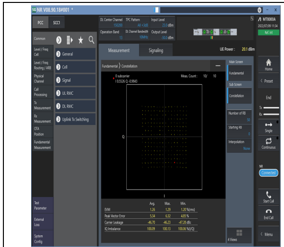
1-N13--15-10-M-5-DFT-256QAM-Outer_Full-50@0-A nt1-see graph-PASS
