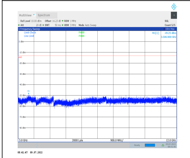
1-N13--15-10-M-1-DFT-PI2BPSK-Inner_1RB_Left-1 @1-3000-12000-Ant1--49.25--13-PASS
