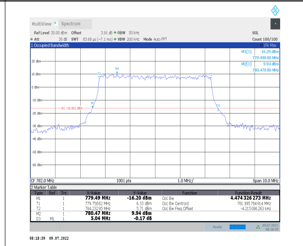
1-N13--15-5-M-7-CP-16QAM-Outer_Full-25@0-Ant1 -4.474-5.040-<math>\leq 5</math>-PASS
