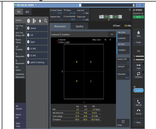
1-N13--15-10-M-6-CP-QPSK-Outer_Full-52@0-Ant 1-see graph-PASS
