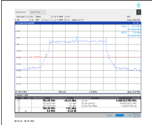
1-N13--15-5-H-9-CP-256QAM-Outer_Full-25@0-Ant 1-4.469-5.000-≤5-PASS
