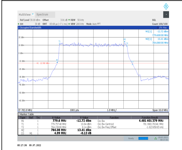
1-N13--15-5-M-2-DFT-PI2BPSK-Outer_Full-25@0-A nt1-4.481-4.990-≤5-PASS
