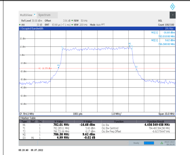
1-N13--15-5-H-6-CP-QPSK-Outer_Full-25@0-Ant1-4 .457-4.990- \leq 5 -PASS
