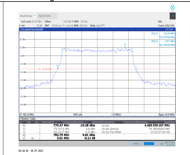
1-N13--15-5-M-5-DFT-256QAM-Outer_Full-25@0-A nt1-4.485-5.010-<math>\leq 5</math>-PASS
