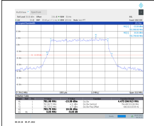
1-N13--15-5-H-5-DFT-256QAM-Outer_Full-25@0-Ant t1-4.473-5.050- \leq 5 -PASS
