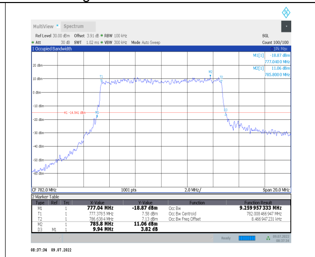
1-N13--15-10-M-7-CP-16QAM-Outer_Full-52@0-Ant1-9.26-9.940-≤10-PASS
