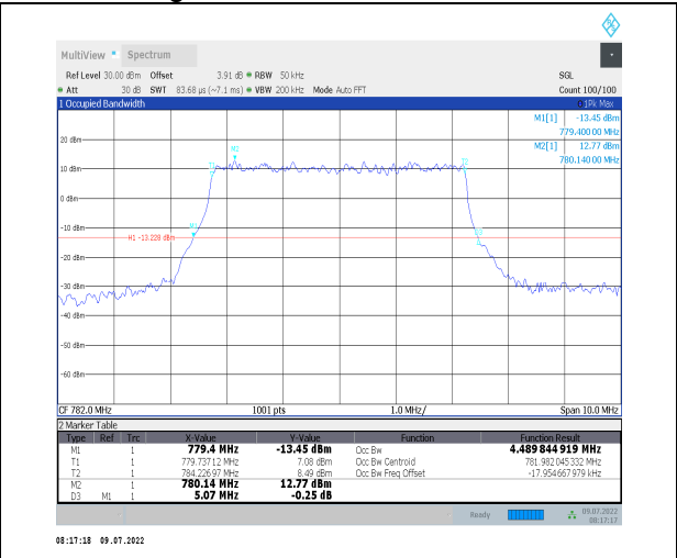
1-N13--15-5-M-1-DFT-QPSK-Outer_Full-25@0-Ant1 -4.49-5.070-≤5-PASS
