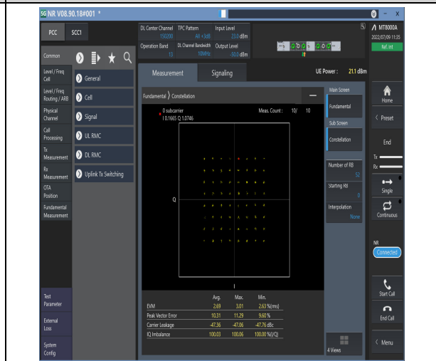
1-N13--15-10-M-8-CP-64QAM-Outer_Full-52@0-Ant1 t1-see graph-PASS
