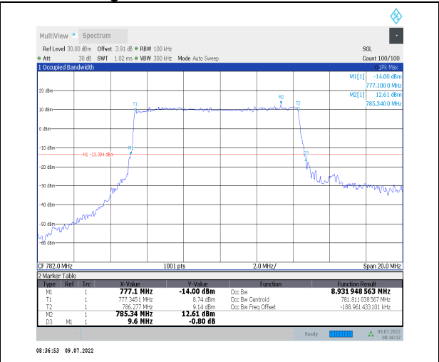
1-N13--15-10-M-3-DFT-16QAM-Outer_Full-50@0-Ant1-8.932-9.600-≤10-PASS
