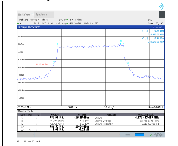
1-N13--15-5-H-8-CP-64QAM-Outer_Full-25@0-Ant1 -4.471-5.050-≤5-PASS
