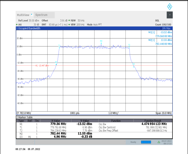
1-N13--15-5-M-3-DFT-16QAM-Outer_Full-25@0-Ant 1-4.475-4.960-≤5-PASS
