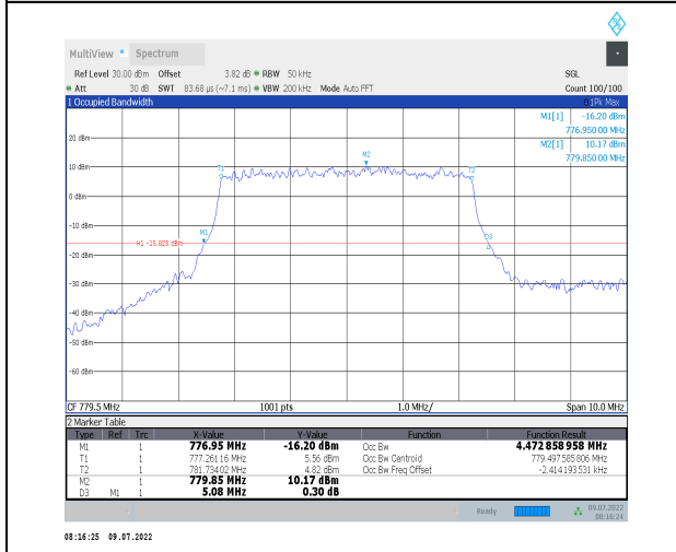
1-N13--15-5-L-7-CP-16QAM-Outer_Full-25@0-Ant1- 4.473-5.080-≤5-PASS
