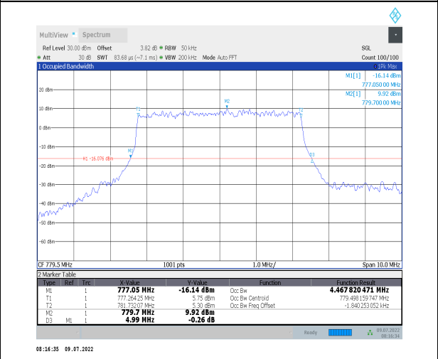
1-N13--15-5-L-8-CP-64QAM-Outer_Full-25@0-Ant1- 4.468-4.990-≤5-PASS
