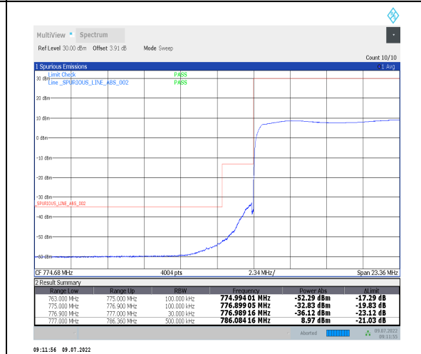
1-N13-PC3-15-10-L-6-CP-QPSK-Outer_Full-52@0-Ant1-PASS-see graph
