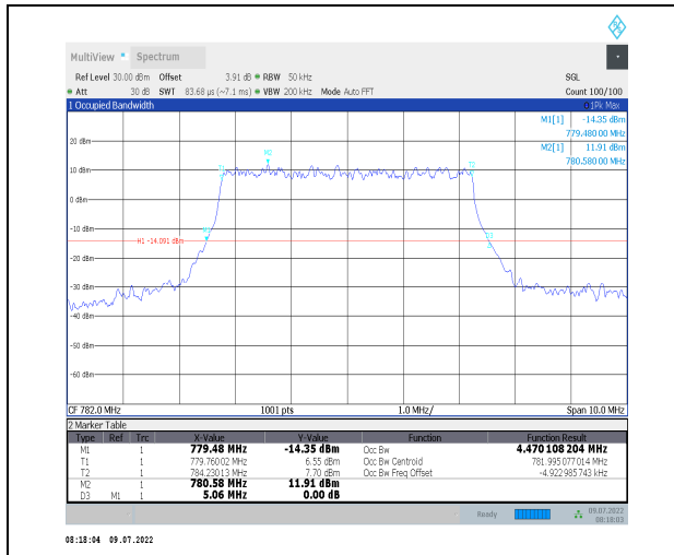
1-N13--15-5-M-4-DFT-64QAM-Outer_Full-25@0-Ant 1-4.47-5.060-<math>\leq 5</math>-PASS
