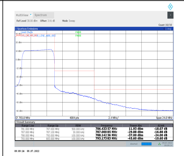
1-N13-PC3-15-5-H-6-CP-QPSK-Outer_Full-25@0-Ant1-PASS-see graph
