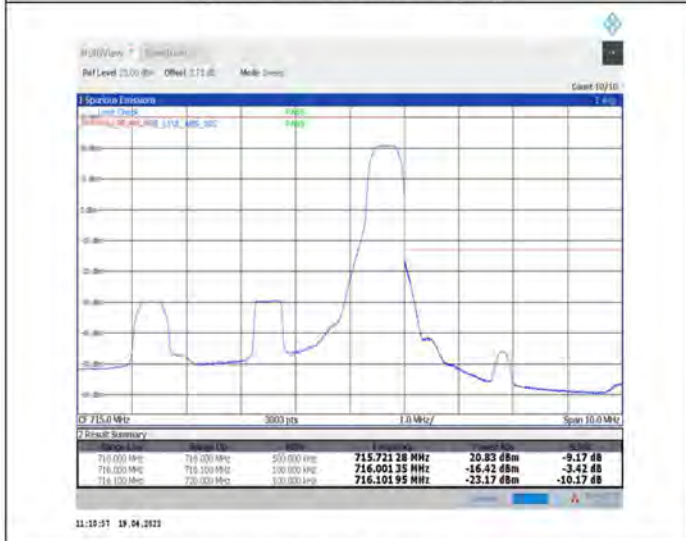
1-N12--15-5-H-5-CP-QPSK-Edge_1RB_Right-1@24-Ant1-PASS-see graph
