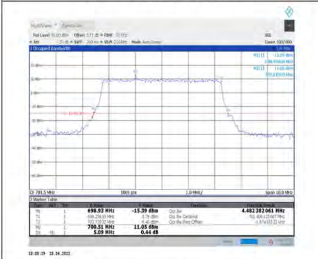
1-N12--15-5-L-7-CP-16QAM-Outer_Full-25@0-Ant1-4.482-5.090-≤5-PASS
