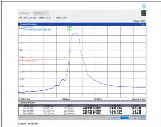
1-N12--15-15-L-1-DFT-PI2BPSK-Edge_1RB_Left-1@0-Ant1-PASS-see graph
