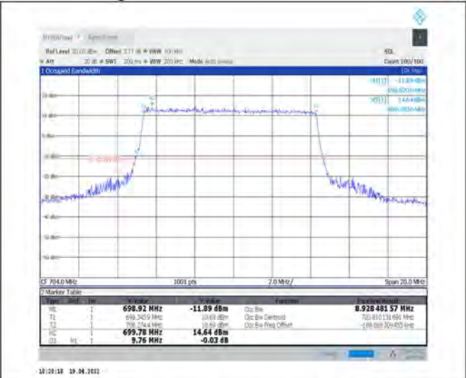
1-N12--15-10-L-3-DFT-16QAM-Outer_Full-50@0-Ant1-8.928-9.760-≤10-PASS
