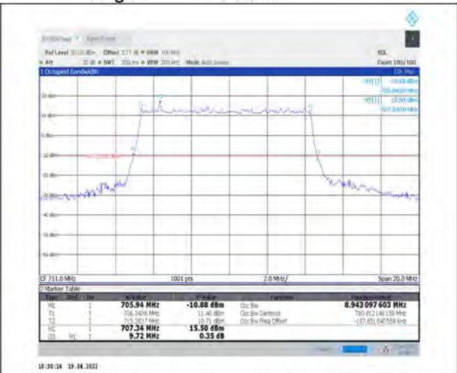
1-N12--15-10-H-1-DFT-QPSK-Outer_Full-50@0-Ant1-8.943-9.720-≤10-PASS
