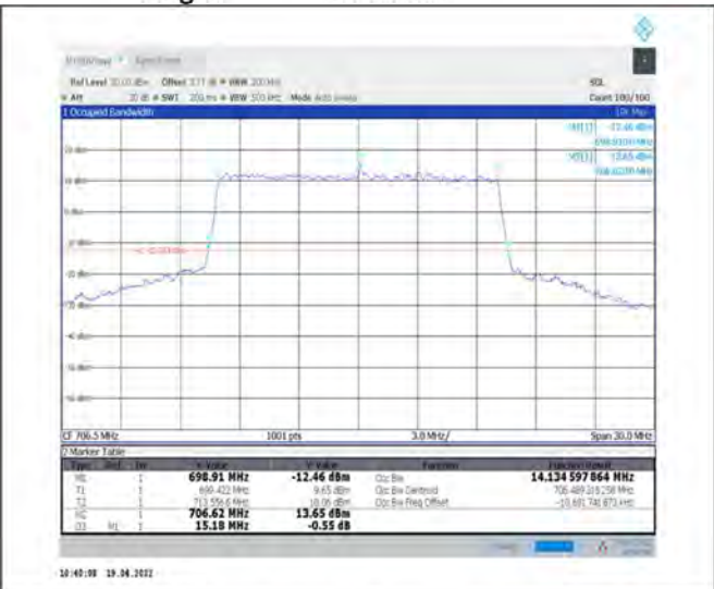
1-N12--15-15-L-8-CP-64QAM-Outer_Full-79@0-Ant1-14.135-15.180-≤15-PASS
