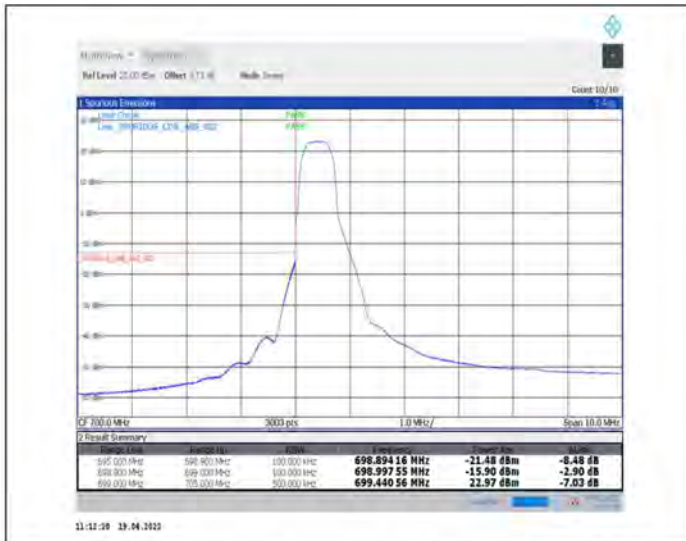
1-N12--15-10-L-1-DFT-PI2BPSK-Edge_1RB_Left-1@0-Ant1-PASS-see graph
