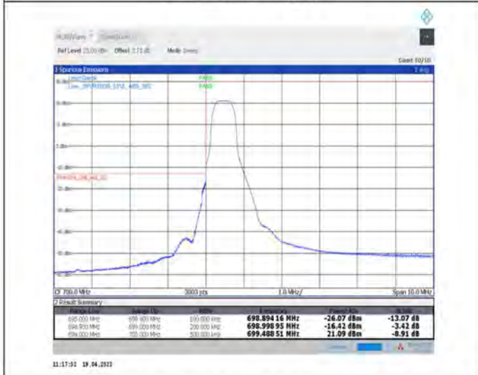
1-N12--15-15-L-4-CP-QPSK-Edge_1RB_Left-1@0-Ant1-PASS-see graph
