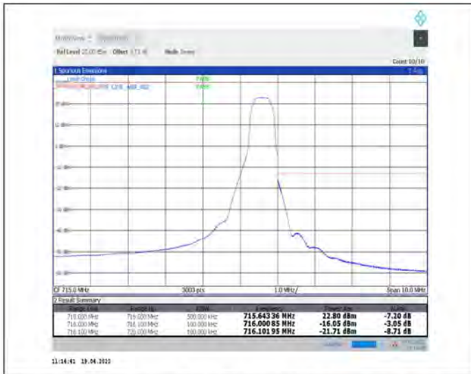
1-N12--15-10-H-2-DFT-PI2BPSK-Edge_1RB_Right-1@51-Ant1-PASS-see graph
