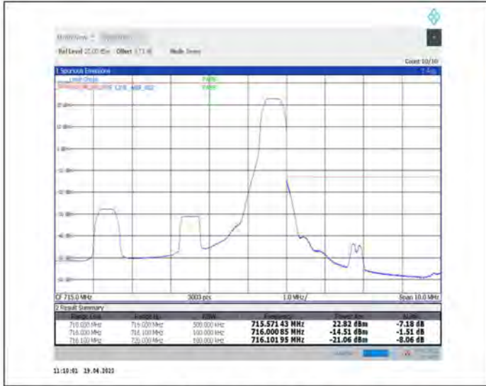
1-N12--15-5-H-2-DFT-PI2BPSK-Edge_1RB_Right-1@24-Ant1-PASS-see graph
