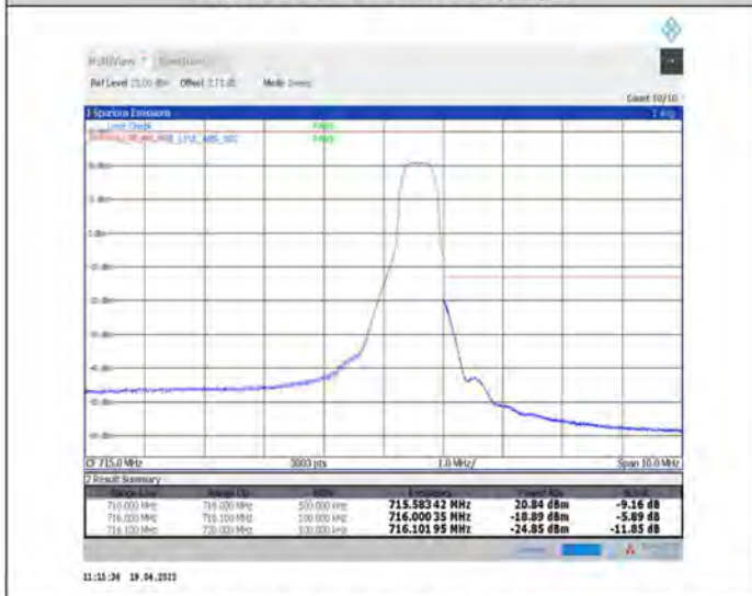
1-N12--15-10-H-5-CP-QPSK-Edge_1RB_Right-1@51-Ant1-PASS-see graph
