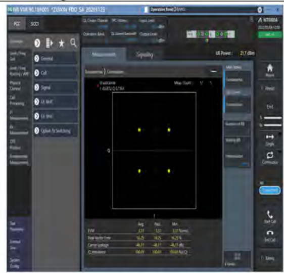
1-N12-PC3-15-15-M-6-CP-QPSK-Outer_Full-79@0-Ant1-see graph-PASS
