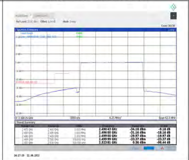
1-N7--15-25-L-6-CP-QPSK-Outer_Full-133@0-Ant1-PASS-see graph
