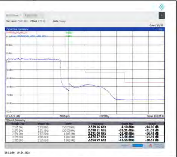
1-N7--15-15-H-3-DFT-PI2BPSK-Outer_Full-75@0-Ant1-PASS-see graph
