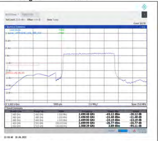
1-N7--15-10-L-3-DFT-PI2BPSK-Outer_Full-50@0-Ant1-PASS-see graph
