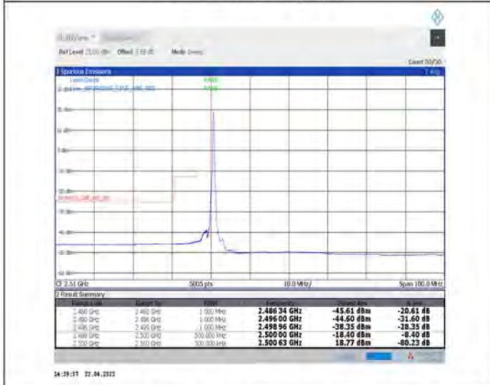
1-N7--15-40-L-4-CP-QPSK-Edge_1RB_Left-1@0-Ant1-PASS-see graph
