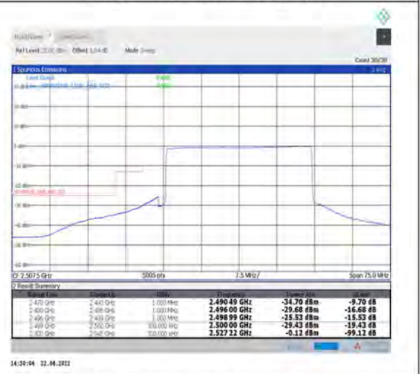
1-N7--15-30-L-6-CP-QPSK-Outer_Full-160@0-Ant1-PASS-see graph
