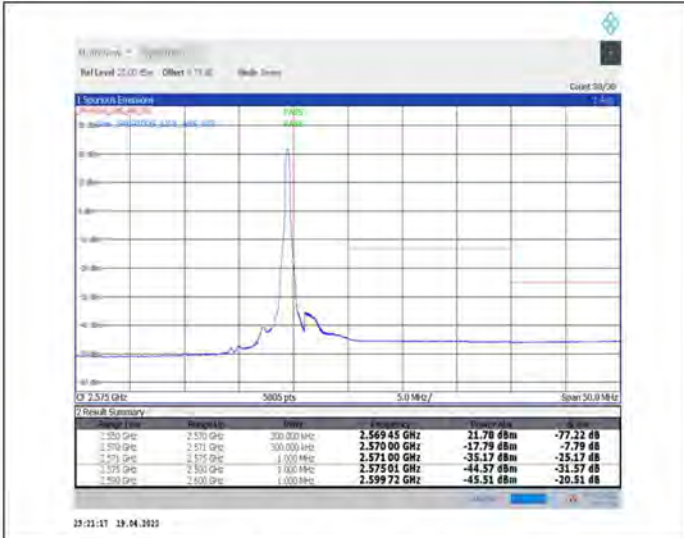
1-N7--15-20-H-2-DFT-PI2BPSK-Edge_1RB_Right-1@105-Ant1-PASS-see graph
