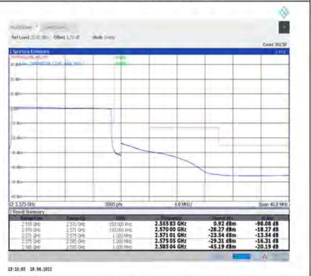
1-N7--15-15-H-6-CP-QPSK-Outer_Full-79@0-Ant1-PASS-see graph
