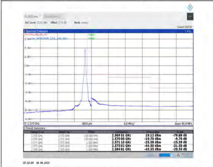
1-N7--15-15-H-5-CP-QPSK-Edge_1RB_Right-1@78-Ant1-PASS-see graph
