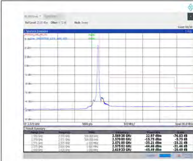
1-N7--15-40-H-2-DFT-PI2BPSK-Edge_1RB_Right-1@215-Ant1-PASS-see graph
