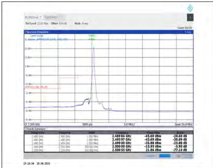
1-N7--15-20-L-1-DFT-PI2BPSK-Edge_1RB_Left-1@0-Ant1-PASS-see graph
