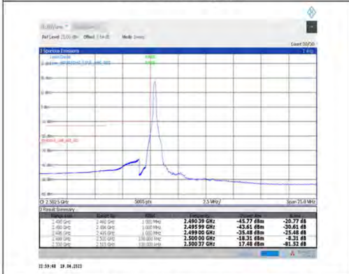
1-N7--15-10-L-4-CP-QPSK-Edge_1RB_Left-1@0-Ant1-PASS-see graph
