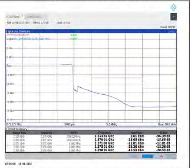
1-N7--15-20-H-6-CP-QPSK-Outer_Full-106@0-Ant1-PASS-see graph
