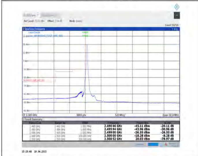
1-N7--15-20-L-4-CP-QPSK-Edge_1RB_Left-1@0-Ant1-PASS-see graph
