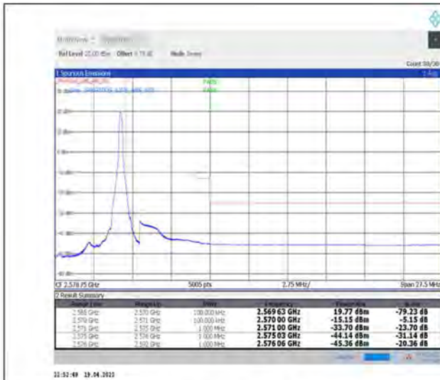
1-N7--15-5-H-2-DFT-PI2BPSK-Edge_1RB_Right-1@24-Ant1-PASS-see graph
