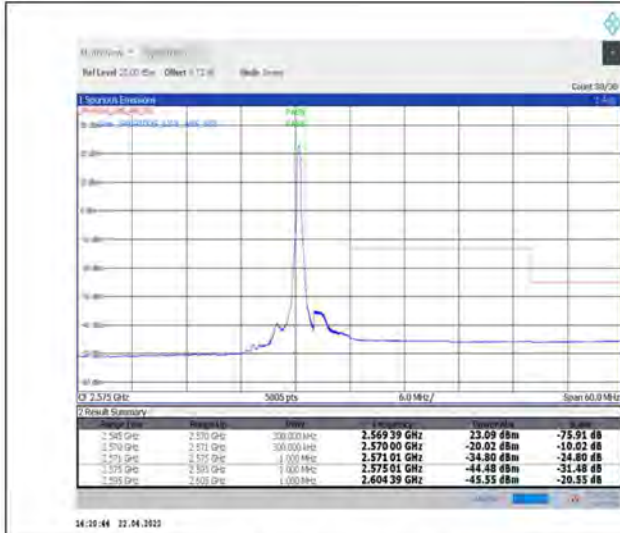
1-N7--15-25-H-2-DFT-PI2BPSK-Edge_1RB_Right-1@132-Ant1-PASS-see graph
