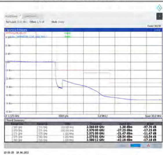
1-N7--15-10-H-6-CP-QPSK-Outer_Full-52@0-Ant1-PASS-see graph
