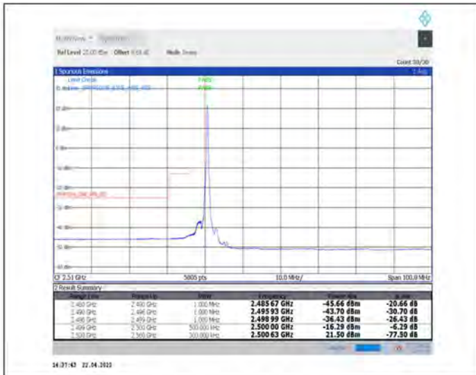
1-N7--15-40-L-1-DFT-PI2BPSK-Edge_1RB_Left-1@0-Ant1-PASS-see graph
