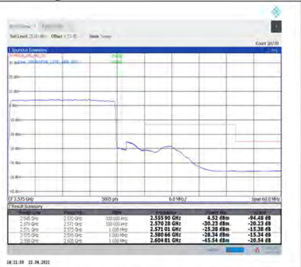
1-N7--15-25-H-3-DFT-PI2BPSK-Outer_Full-128@0-Ant1-PASS-see graph
