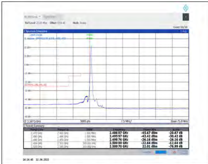
1-N7--15-30-L-1-DFT-PI2BPSK-Edge_1RB_Left-1@0-Ant1-PASS-see graph
