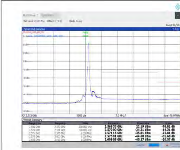
1-N7--15-30-H-2-DFT-PI2BPSK-Edge_1RB_Right-1@159-Ant1-PASS-see graph
