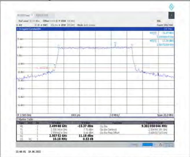
1-N7--15-10-L-7-CP-16QAM-Outer_Full-52@0-Ant1-9.302-10.180-≤10-PASS
