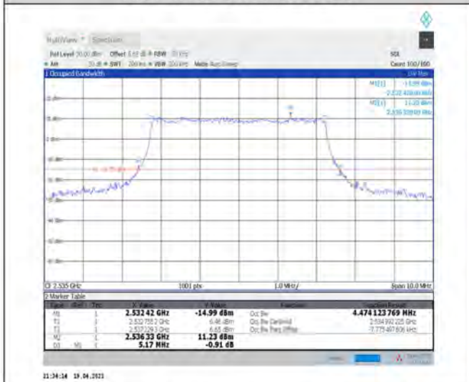
1-N7--15-5-M-6-CP-QPSK-Outer_Full-25@0-Ant1-4.474-5.170-≤5-PASS
