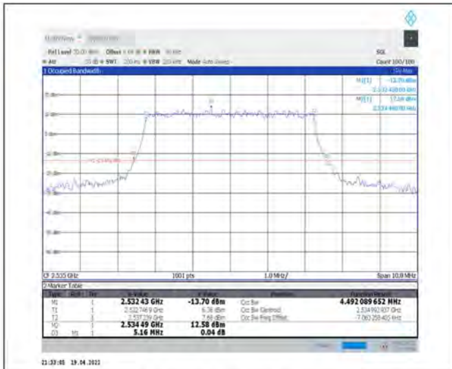
1-N7--15-5-M-4-DFT-64QAM-Outer_Full-25@0-Ant1-4.492-5.160-≤5-PASS
