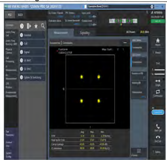
1-N7-PC3-15-40-M-6-CP-QPSK-Outer_Full-216@0-Ant1-see graph-PASS
