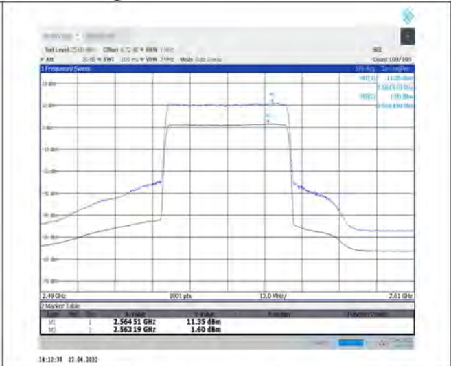
1-N7--15-40-H-2-CP-256QAM-Outer_Full-216@0- Ant1-9.75-100%-0.00-9.75-PASS-≤13
