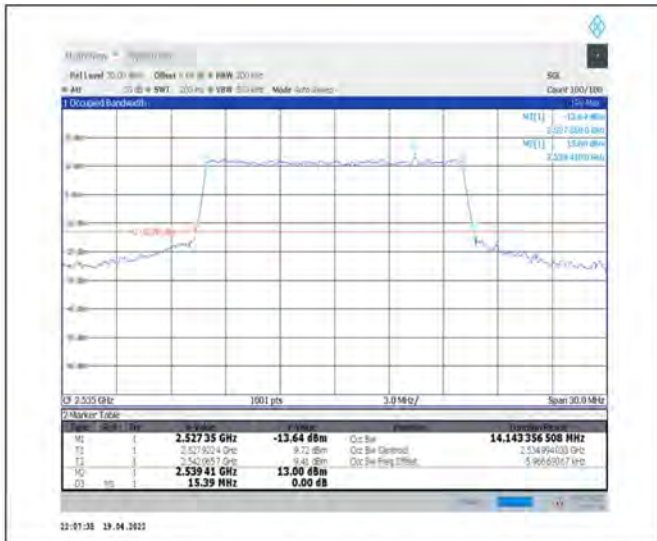
1-N7--15-15-M-6-CP-QPSK-Outer_Full-79@0-Ant1-14.143-15.390-≤15-PASS
