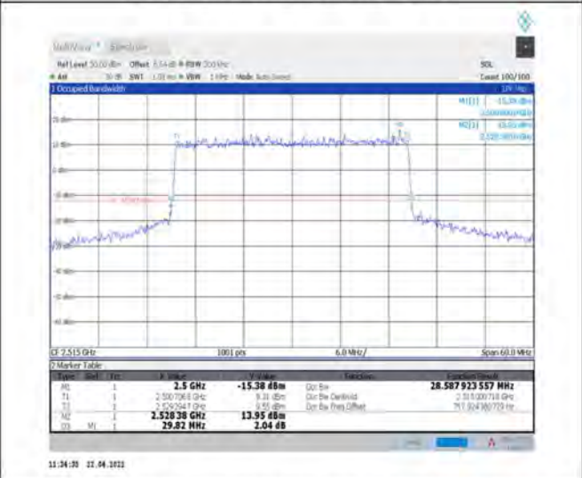
1-N7--15-30-L-1-DFT-QPSK-Outer_Full-160@0-Ant1-28.589-29.820-≤30-PASS
