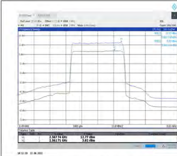
1-N7--15-40-H-1-DFT-256QAM-Outer_Full-216@0- Ant1-8.95-100%-0.00-8.95-PASS-≤13
