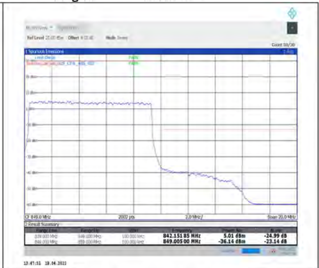
1-N5--15-10-H-3-DFT-PI2BPSK-Outer_Full-50@0-Ant1-seegraph-PASS-see graph
