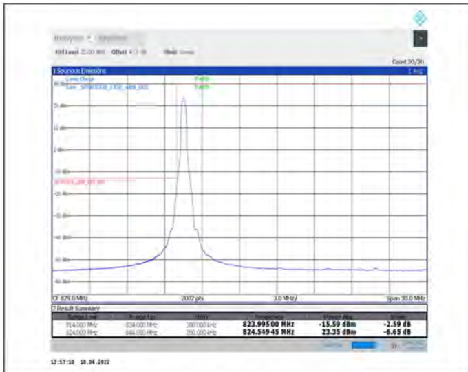
1-N5--15-20-L-1-DFT-PI2BPSK-Edge_1RB_Left-1@0-Ant1-seegraph-PASS-see graph
