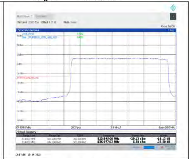
1-N5--15-20-L-3-DFT-PI2BPSK-Outer_Full-100@0-Ant1-seegraph-PASS-see graph
