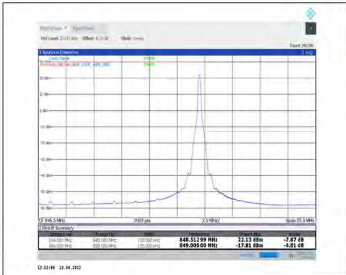
1-N5--15-15-H-2-DFT-PI2BPSK-Edge_1RB_Right-1@78-Ant1-seegraph-PASS-see graph
