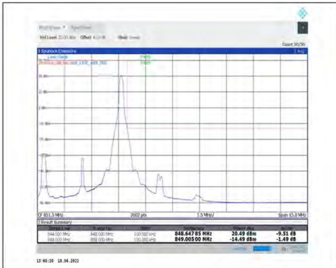
1-N5--15-5-H-2-DFT-PI2BPSK-Edge_1RB_Right-1@24-Ant1-seegraph-PASS-see graph
