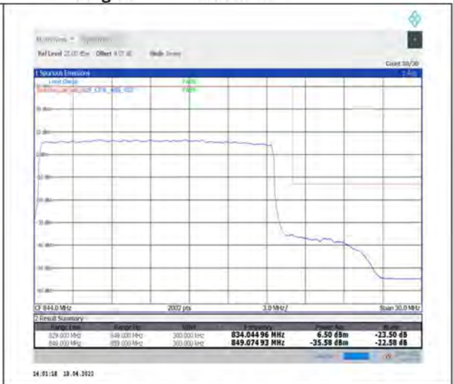
1-N5--15-20-H-3-DFT-PI2BPSK-Outer_Full-100@0-Ant1-seegraph-PASS-see graph
