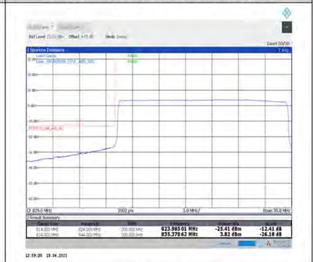
1-N5--15-20-L-6-CP-QPSK-Outer_Full-106@0-Ant1-seegraph-PASS-see graph
