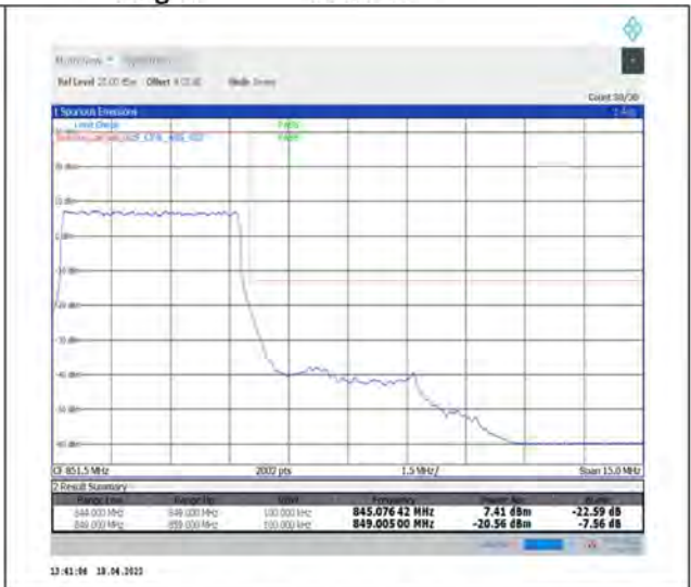
1-N5--15-5-H-3-DFT-PI2BPSK-Outer_Full-25@0-Ant1-seegraph-PASS-see graph
