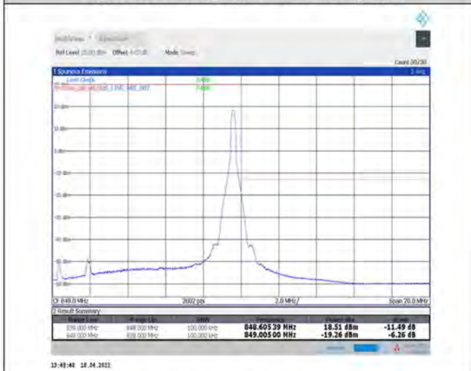
1-N5--15-10-H-5-CP-QPSK-Edge_1RB_Right-1@51-Ant1-seegraph-PASS-see graph
