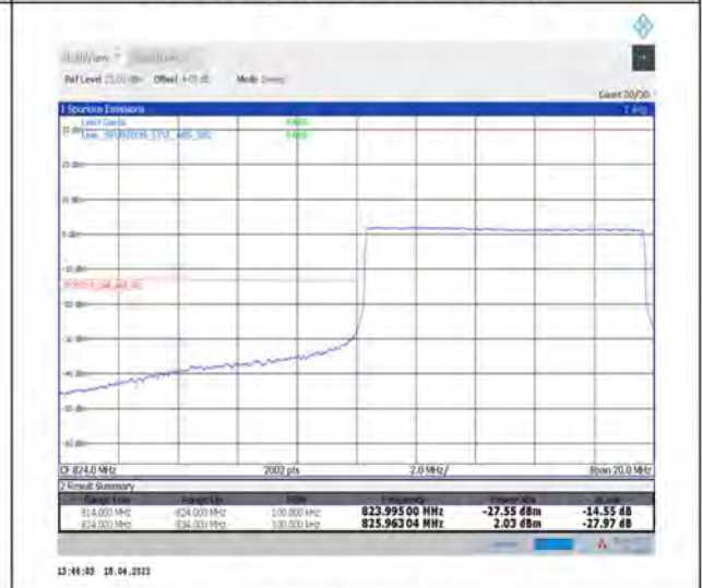
1-N5--15-10-L-6-CP-QPSK-Outer_Full-52@0-Ant1-seegraph-PASS-see graph
