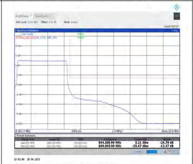
1-N5--15-5-H-6-CP-QPSK-Outer_Full-25@0-Ant1-seegraph-PASS-see graph
