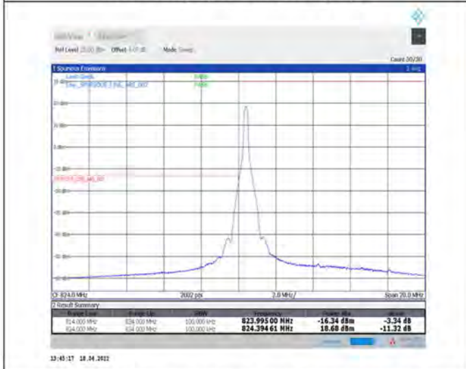
1-N5--15-10-L-4-CP-QPSK-Edge_1RB_Left-1@0-Ant1-seegraph-PASS-see graph
