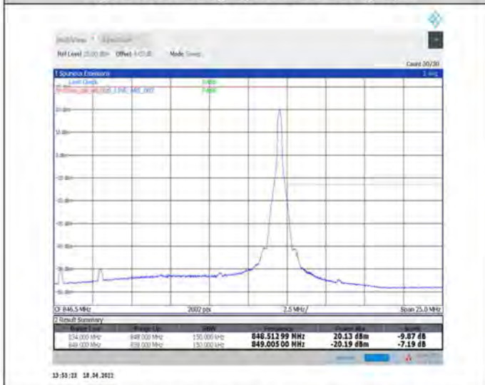
1-N5--15-15-H-5-CP-QPSK-Edge_1RB_Right-1@78-Ant1-seegraph-PASS-see graph
