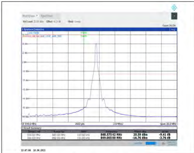
1-N5--15-10-H-2-DFT-PI2BPSK-Edge_1RB_Right-1@51-Ant1-seegraph-PASS-see graph
