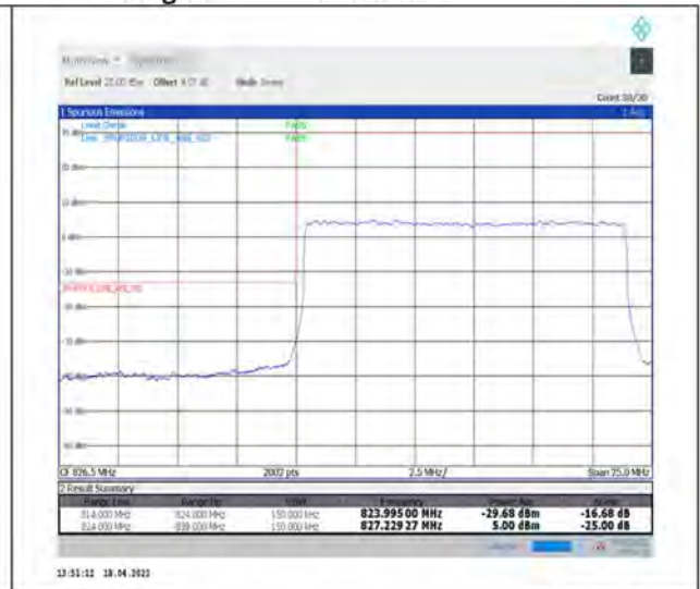
1-N5--15-15-L-3-DFT-PI2BPSK-Outer_Full-75@0-Ant1-seegraph-PASS-see graph
