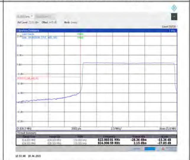
1-N5--15-15-L-6-CP-QPSK-Outer_Full-79@0-Ant1-seegraph-PASS-see graph
