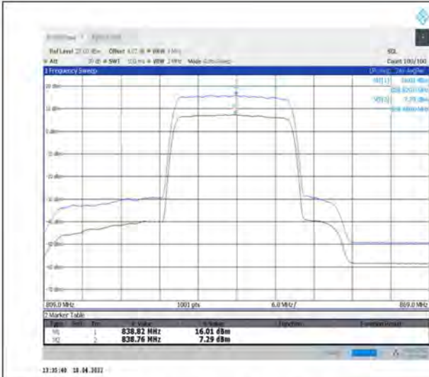
1-N5--15-20-H-1-DFT-256QAM-Outer_Full-100@0- Ant1-8.72-100%-0.00-8.72-PASS-≤13
