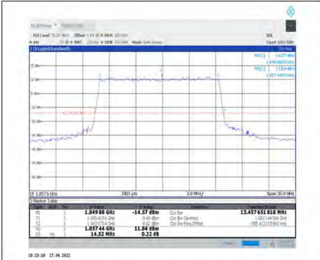
1-N2--15-15-L-3-DFT-16QAM-Outer_Full-75@0-Ant1-13.458-14.520-≤15-PASS
