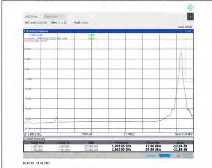
1-N2--15-20-H-5-CP-QPSK-Edge_1RB_Right-1@105-Ant1-seegraph-PASS-see graph
