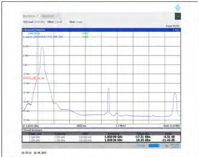
1-N2--15-10-L-1-DFT-PI2BPSK-Edge_1RB_Left-1@0-Ant1-seegraph-PASS-see graph
