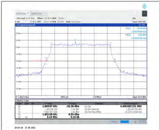
1-N2--15-5-L-9-CP-256QAM-Outer_Full-25@0-Ant1- 4.491-5.190-≤5-PASS
