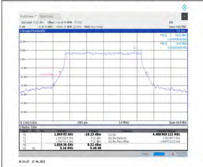
1-N2--15-5-L-7-CP-16QAM-Outer_Full-25@0-Ant1-4.489-5.160-≤5-PASS
