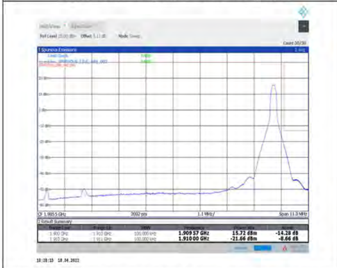
1-N2--15-10-H-5-CP-QPSK-Edge_1RB_Right-1@51-Ant1-seegraph-PASS-see graph
