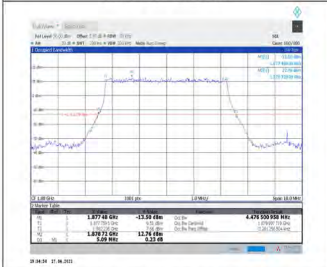
1-N2--15-5-M-2-DFT-PI2BPSK-Outer_Full-25@0- Ant1-4.477-5.090-≤5-PASS
