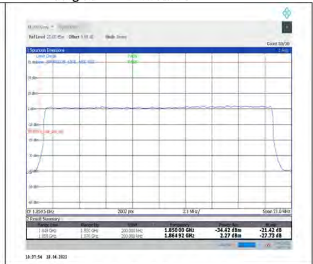
1-N2--15-20-L-3-DFT-PI2BPSK-Outer_Full-100@0-Ant1-seegraph-PASS-see graph
