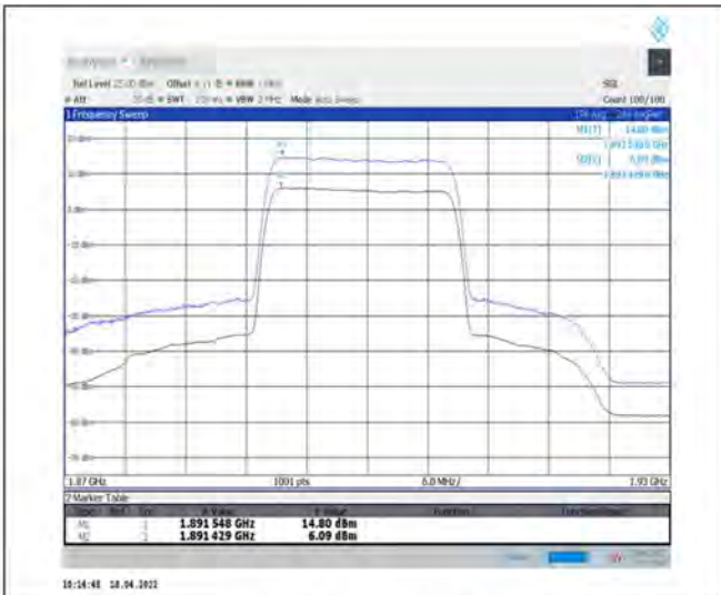
1-N2--15-20-H-1-DFT-256QAM-Outer_Full-100@0- Ant1-8.71-100%-0.00-8.71-PASS-≤13
