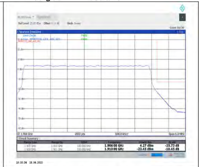
1-N2--15-5-H-3-DFT-PI2BPSK-Outer_Full-25@0-Ant1-seegraph-PASS-see graph
