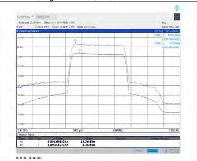
1-N2--15-20-H-2-CP-256QAM-Outer_Full-106@0- Ant1-10.00-100%-0.00-10.00-PASS-≤13
