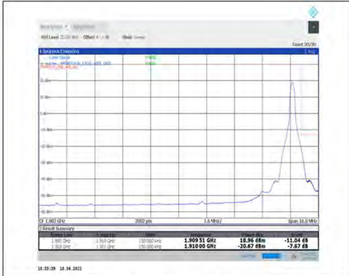
1-N2--15-15-H-2-DFT-PI2BPSK-Edge_1RB_Right-1@78-Ant1-seegraph-PASS-see graph
