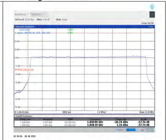
1-N2--15-10-L-3-DFT-PI2BPSK-Outer_Full-50@0-Ant1-seegraph-PASS-see graph
