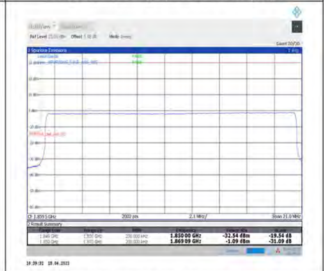
1-N2--15-20-L-6-CP-QPSK-Outer_Full-106@0-Ant1-seegraph-PASS-see graph
