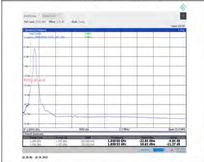
1-N2--15-20-L-4-CP-QPSK-Edge_1RB_Left-1@0-Ant1-seegraph-PASS-see graph
