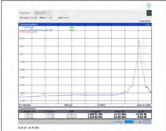
1-N2--15-15-H-5-CP-QPSK-Edge_1RB_Right-1@78-Ant1-seegraph-PASS-see graph
