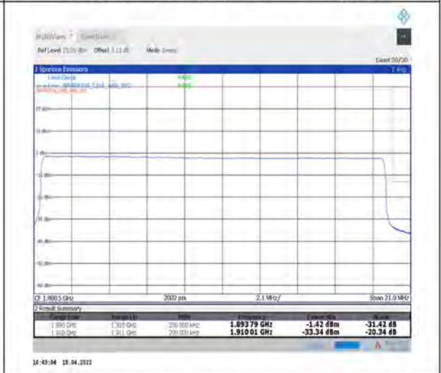
1-N2--15-20-H-6-CP-QPSK-Outer_Full-106@0-Ant1-seegraph-PASS-see graph
