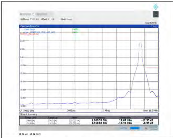
1-N2--15-10-H-2-DFT-PI2BPSK-Edge_1RB_Right-1@51-Ant1-seegraph-PASS-see graph
