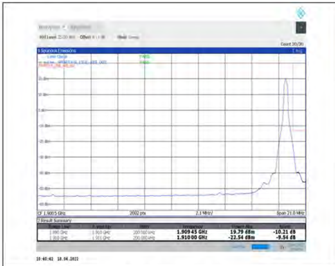
1-N2--15-20-H-2-DFT-PI2BPSK-Edge_1RB_Right-1@105-Ant1-seegraph-PASS-see graph
