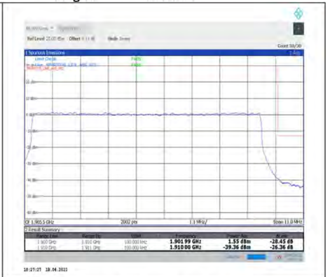
1-N2--15-10-H-3-DFT-PI2BPSK-Outer_Full-50@0-Ant1-seegraph-PASS-see graph
