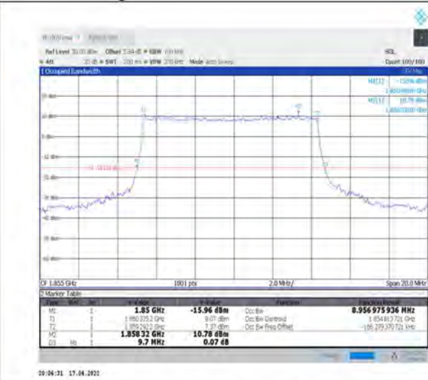
1-N2--15-10-L-3-DFT-16QAM-Outer_Full-50@0-Ant1-8.957-9.700-≤10-PASS
