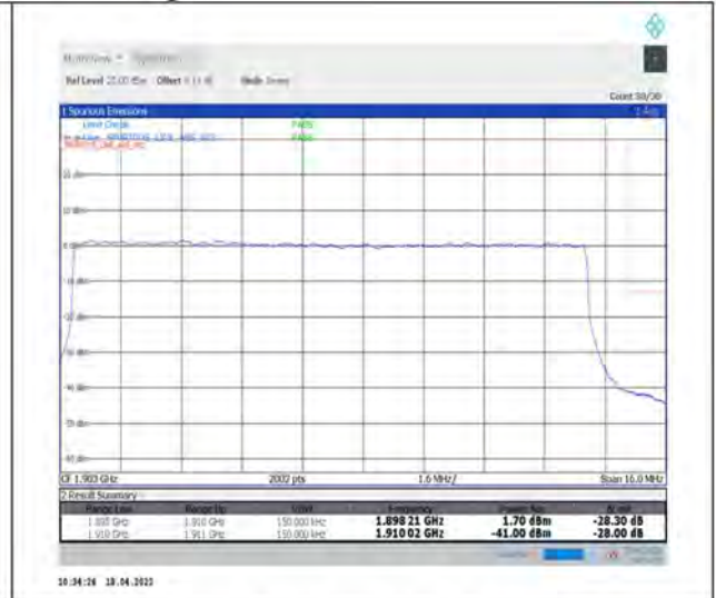
1-N2--15-15-H-3-DFT-PI2BPSK-Outer_Full-75@0-Ant1-seegraph-PASS-see graph
