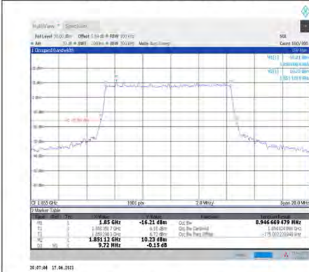
1-N2--15-10-L-4-DFT-64QAM-Outer_Full-50@0-Ant1-8.947-9.720-≤10-PASS
