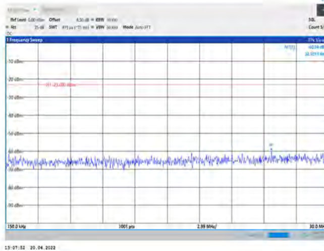
5-5-10MHz-10MHz-QPSK-QPSK-20450-20549-1RB#0-0RB#0-0.15~30MHz
