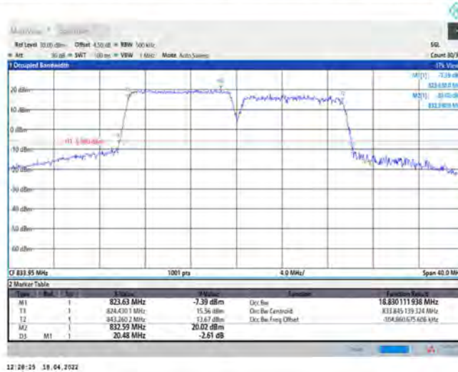
5-5-10MHz-10MHz-QPSK-QPSK-20476-20575-50RB#0-50RB#0
