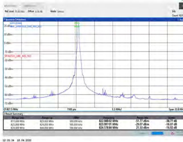
5-5-10MHz-10MHz-QPSK-QPSK-20450-20549-50RB#0-50RB#0
