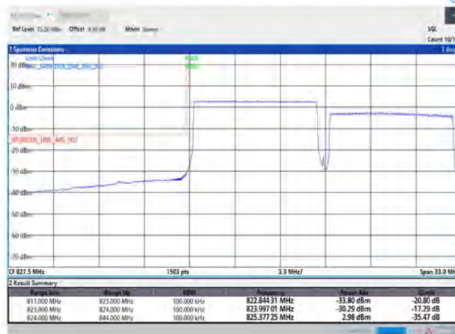
5-5-10MHz-10MHz-QPSK-QPSK-20450-20549-50RB#0-50RB#0
