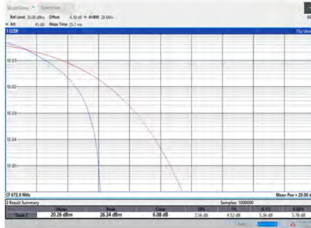
Band71-20MHz-QPSK-133322-100RB#0
