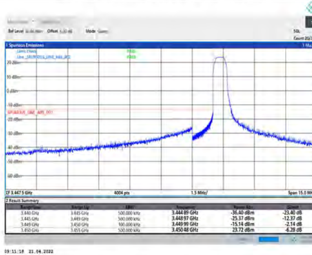
Band42-5MHz-QPSK-42115-25RB#0
