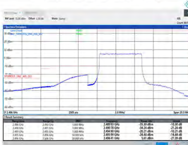
Band41-5MHz-QPSK-39675-25RB#0
