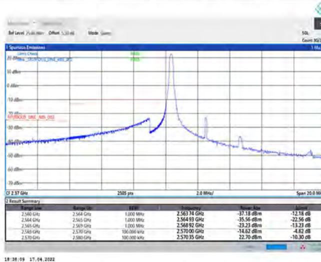
Band38-5MHz-QPSK-37775-25RB#0
