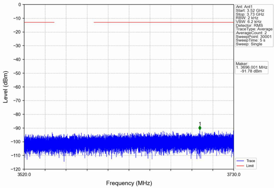
n48_30kHz_SISO_NTNV_40MHz_DFT-s-OFDM_QPSK_3570MHz_Edge_1RB_Left
