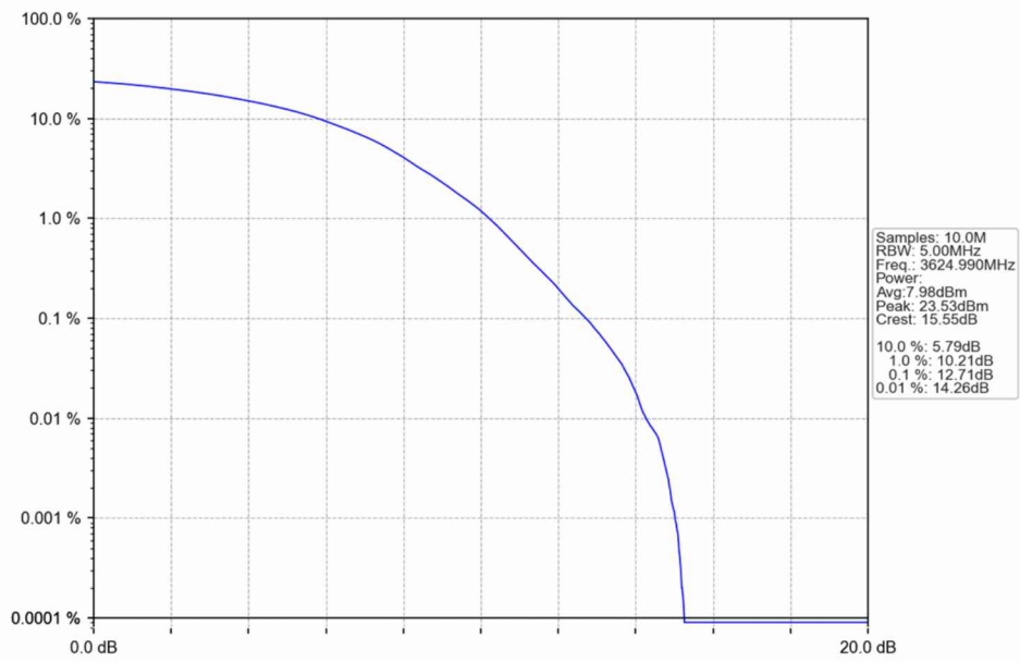
n48_30kHz_SISO_NTNV_40MHz_DFT-s-OFDM_64_QAM_3624.99MHz_Outer_Full
