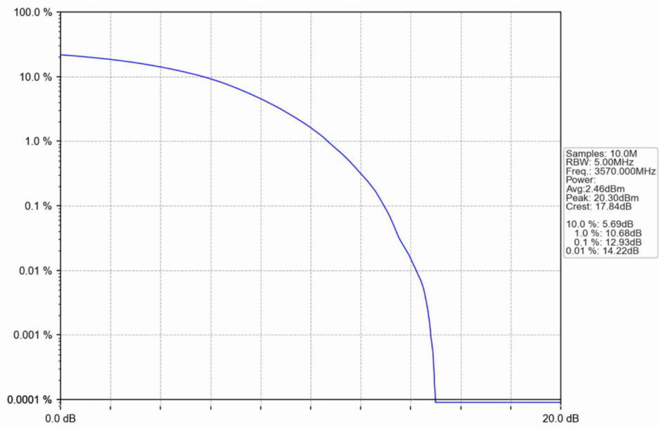
n48_30kHz_SISO_NTNV_40MHz_CP-OFDM_256_QAM_3570MHz_Outer_Full
