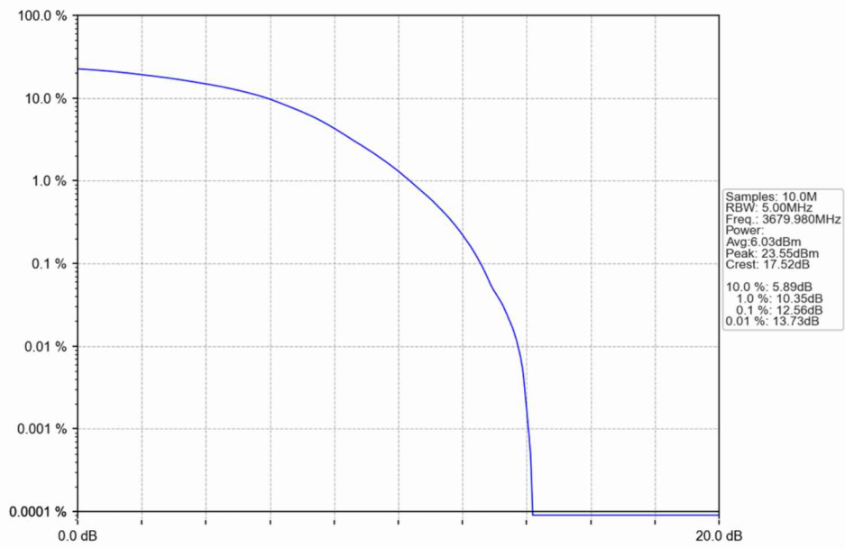
n48_30kHz_SISO_NTNV_40MHz_DFT-s-OFDM_256_QAM_3679.98MHz_Outer_Full
