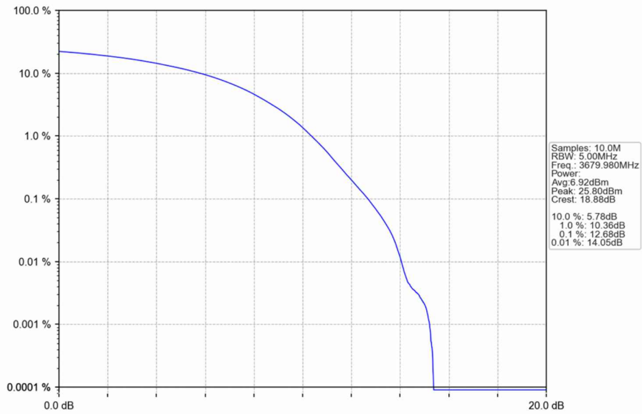
n48_30kHz_SISO_NTNV_40MHz_CP-OFDM_64_QAM_3679.98MHz_Outer_Full
