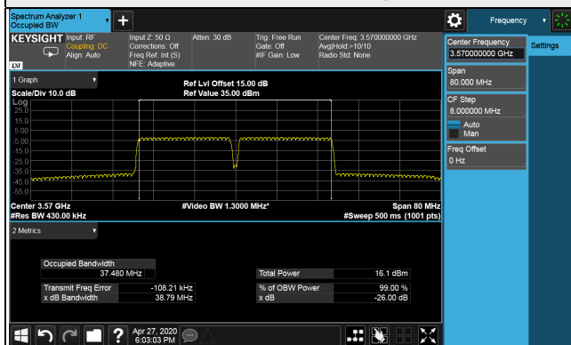
99% Occupied Bandwidth Spectrum Plot of Worst Value 20MHz+20MHz / 16QAM
