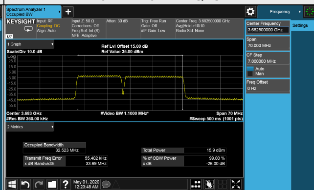
26dB Bandwidth Spectrum Plot of Worst Value 15MHz+20MHz / QPSK
