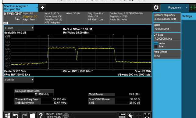
99% Occupied Bandwidth Spectrum Plot of Worst Value 15MHz+20MHz / 16QAM
