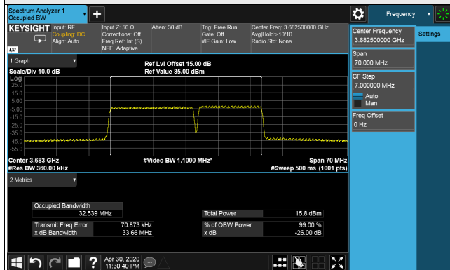
99% Occupied Bandwidth Spectrum Plot of Worst Value 20MHz+15MHz / 16QAM
