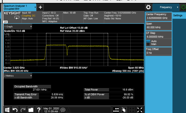
26dB Bandwidth Spectrum Plot of Worst Value 10MHz+20MHz / QPSK
