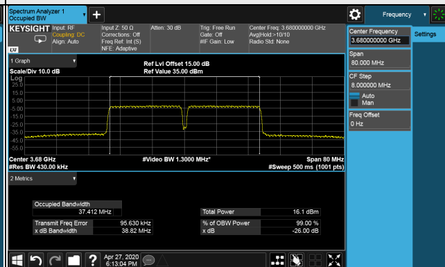
26dB Bandwidth Spectrum Plot of Worst Value 20MHz+20MHz / 64QAM
