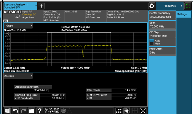
26dB Bandwidth Spectrum Plot of Worst Value 20MHz+15MHz / 16QAM
