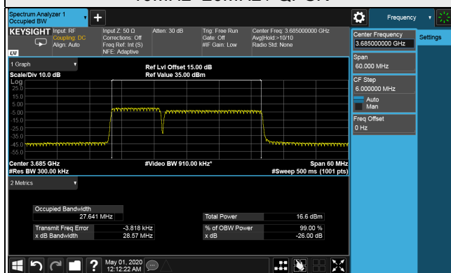
99% Occupied Bandwidth Spectrum Plot of Worst Value 10MHz+20MHz / QPSK
