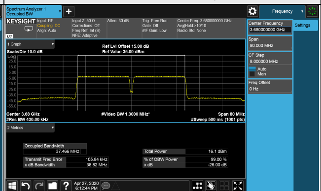
26dB Bandwidth Spectrum Plot of Worst Value 20MHz+20MHz / 16QAM
