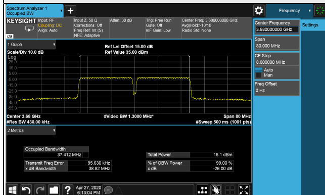
99% Occupied Bandwidth Spectrum Plot of Worst Value 20MHz+20MHz / 64QAM
