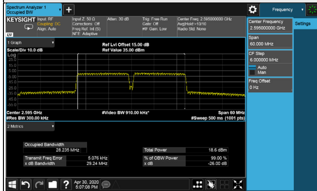
99% Occupied Bandwidth Spectrum Plot of Worst Value 15MHz+15MHz / 64QAM
