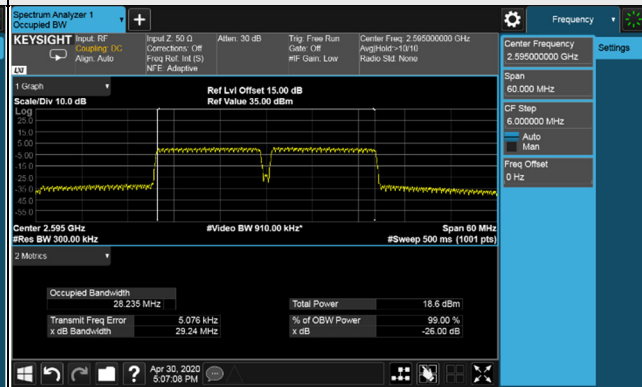
26dB Bandwidth Spectrum Plot of Worst Value 15MHz+15MHz / 64QAM
