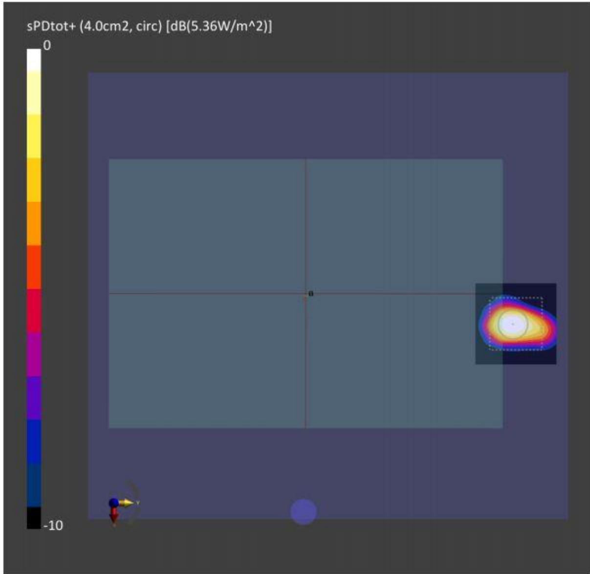
Figure 8-4: 4cm 2 -averaged power density distribution measured at input.power.limit of 5.36 dBm on the Right Side for n261 beam 29
