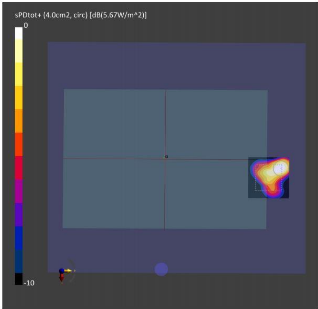
Figure 8-3: 4cm 2 -averaged power density distribution measured at input.power.limit of 5.67 dBm on the Bottom surface for n260 beam 30
