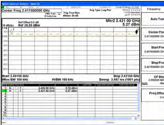
2402-2421MHz
