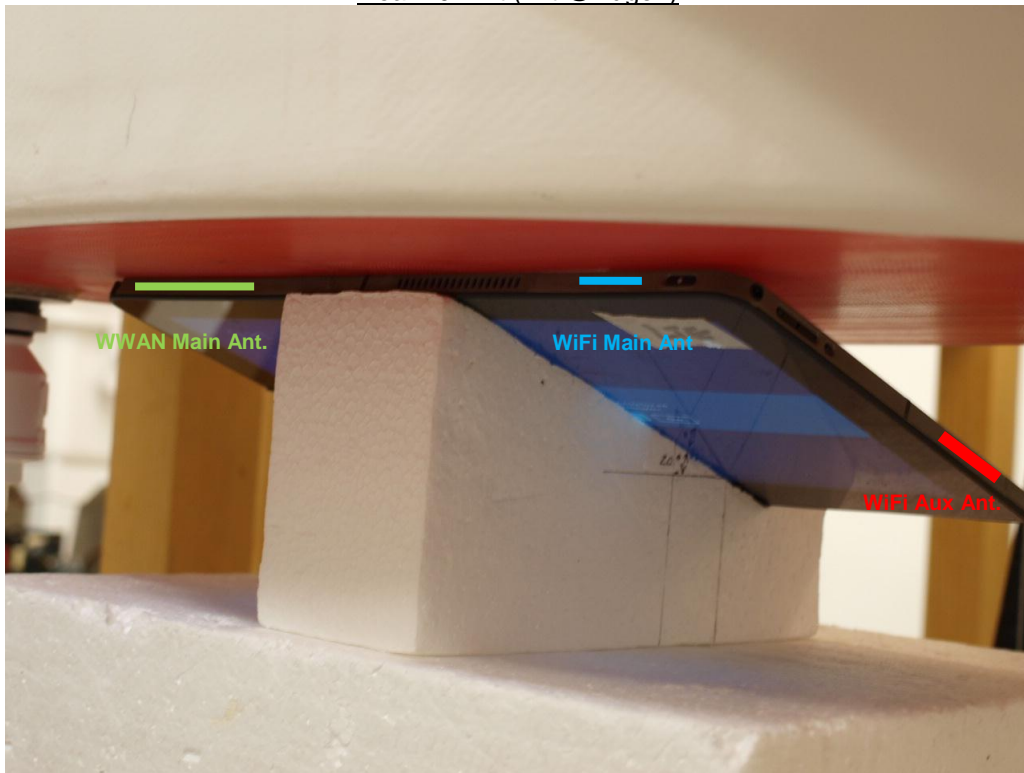
Rear 20° Tilt (Tilt @Edge2)
