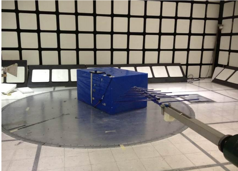
Test Setup
