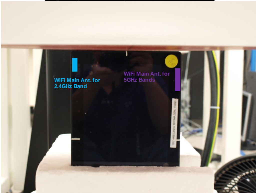
Body – Edge2 w/ 0 mm Separation for WiFi 2.4GHz Band
