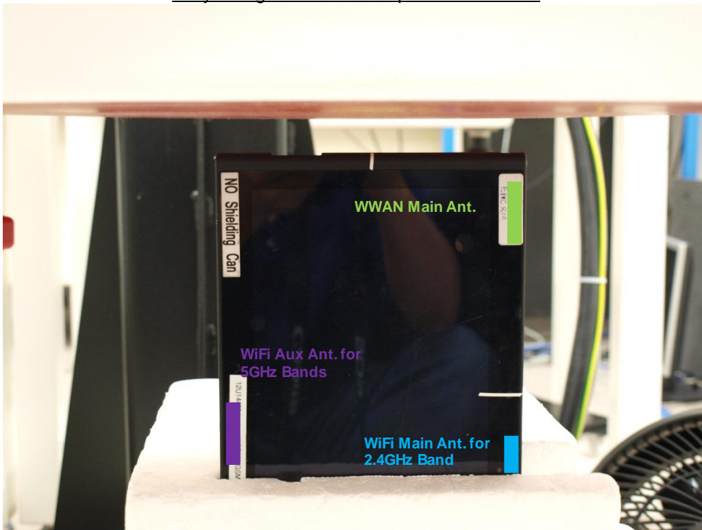
Body – Rear/Bottom (20° Tilt @Edge3 for WiFi 5GHz Bands)
