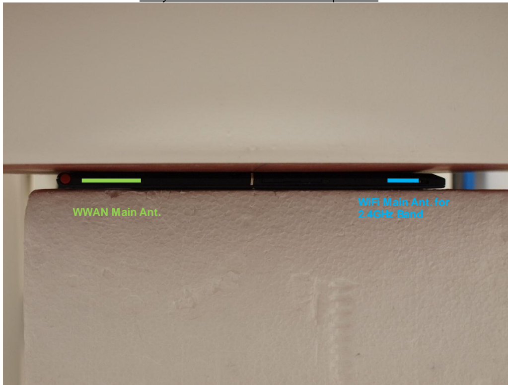
Body – Rear/Bottom (20° Tilt @Edge1 for GSM/UMTS/WiFi 2.4)
