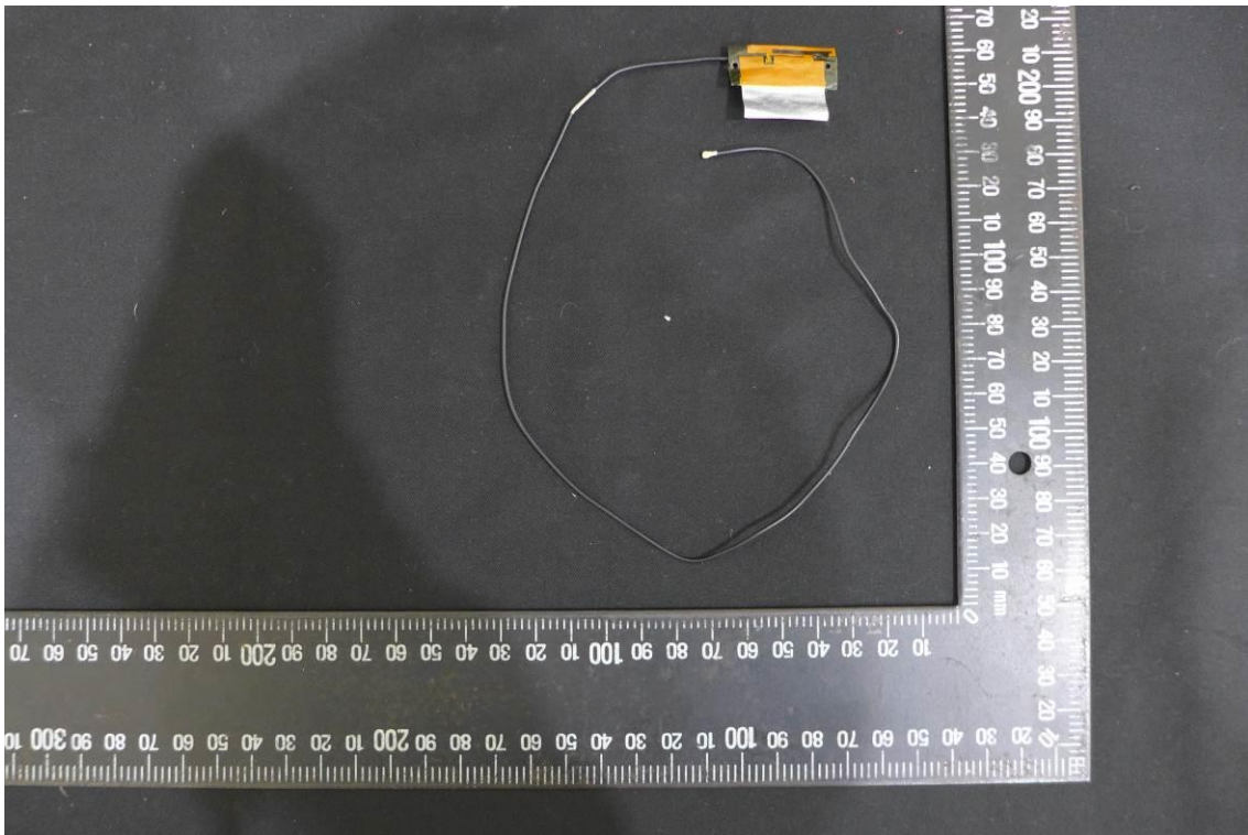
Antenna: AWAN/025.901U8.0001
