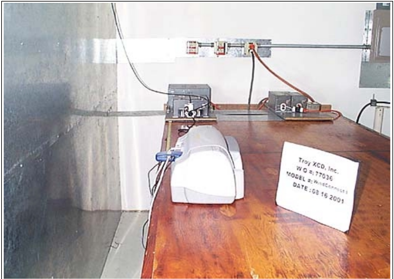
Mains Conducted Emissions - Back View (Brea Setup)
