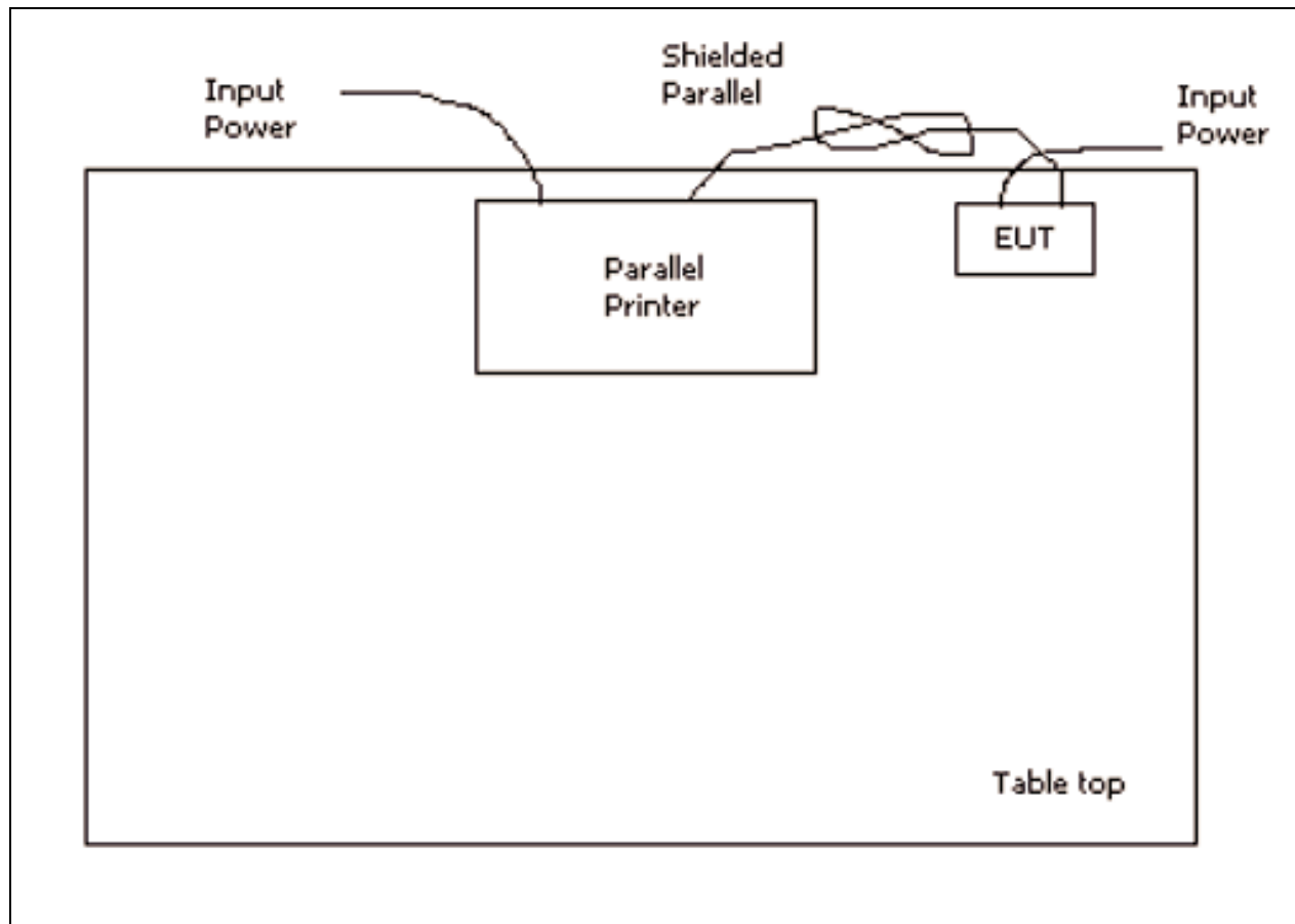
Conducted Emissions
