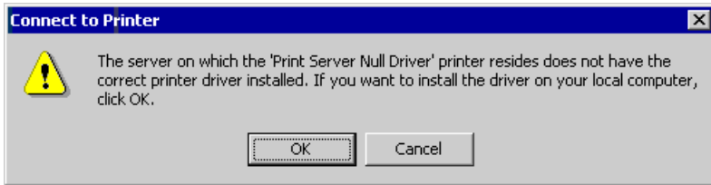
Figure 42: Windows 2000 Message
