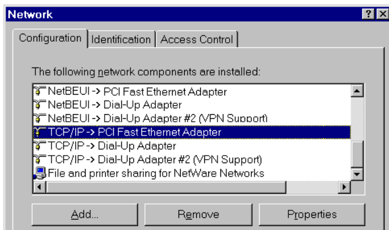
Figure 3: Network Configuration
