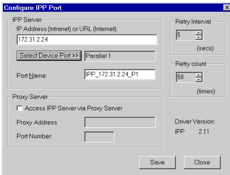
Figure 35: IPP Port
