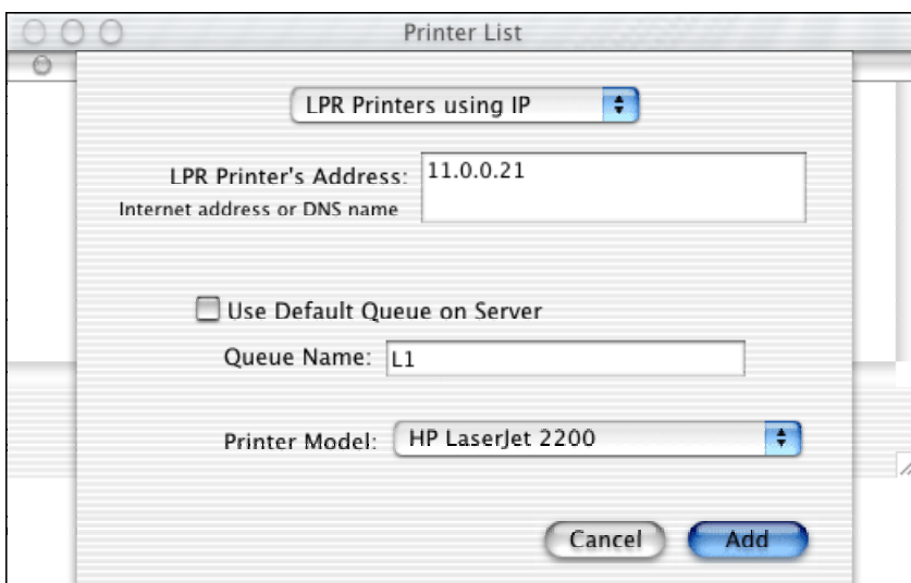
Figure 18: LPR Screen
