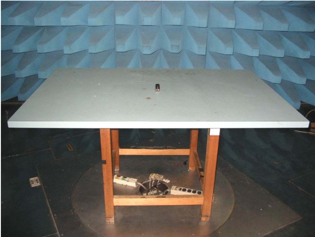
Front View of the Test Configuration (X-plane)
