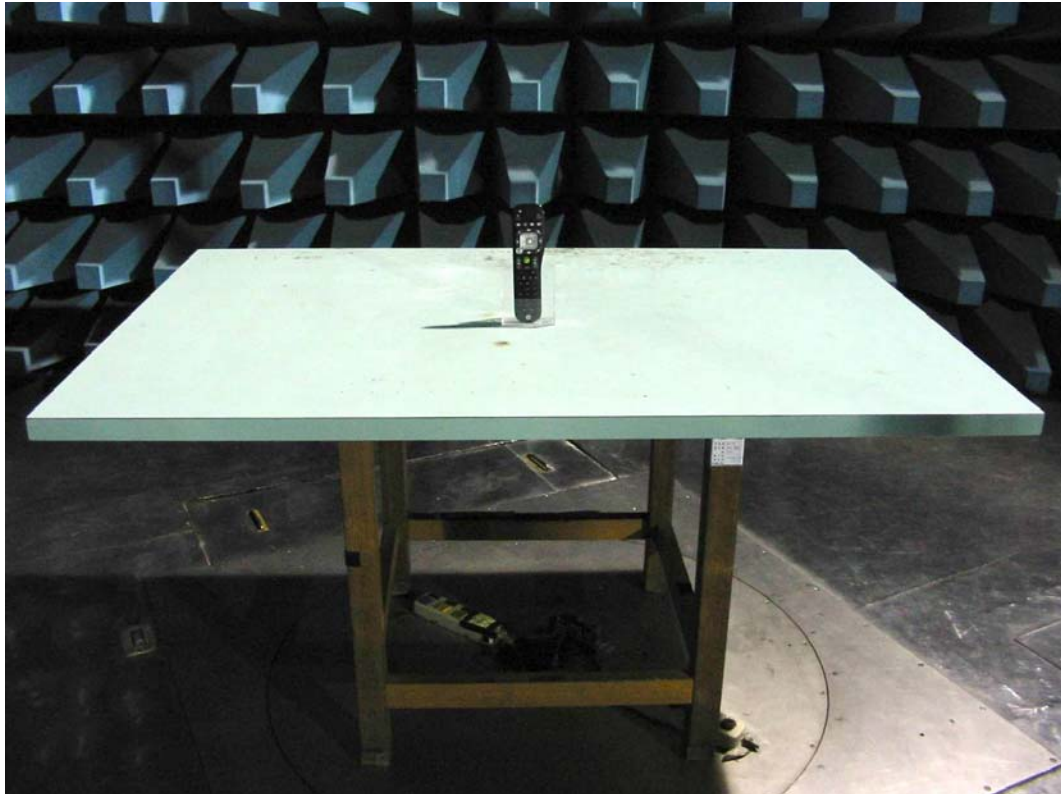
Front View of the Test Configuration (Y-plane)
