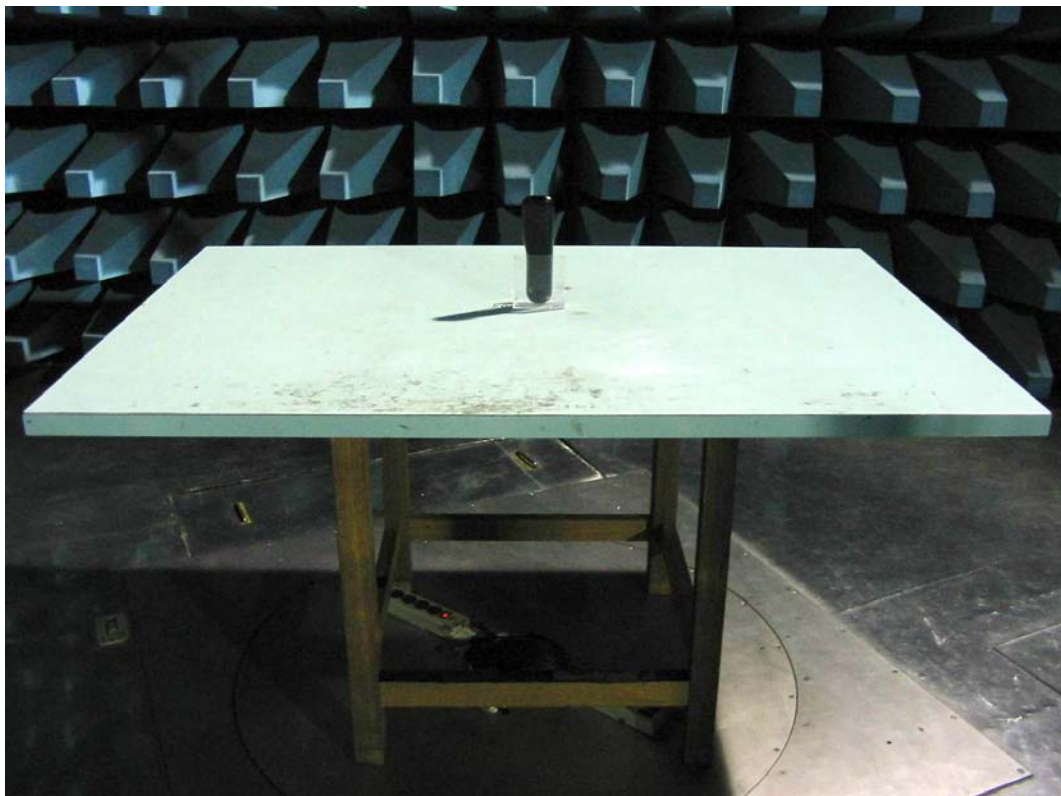
Rear View of the Test Configuration (Y-plane)
