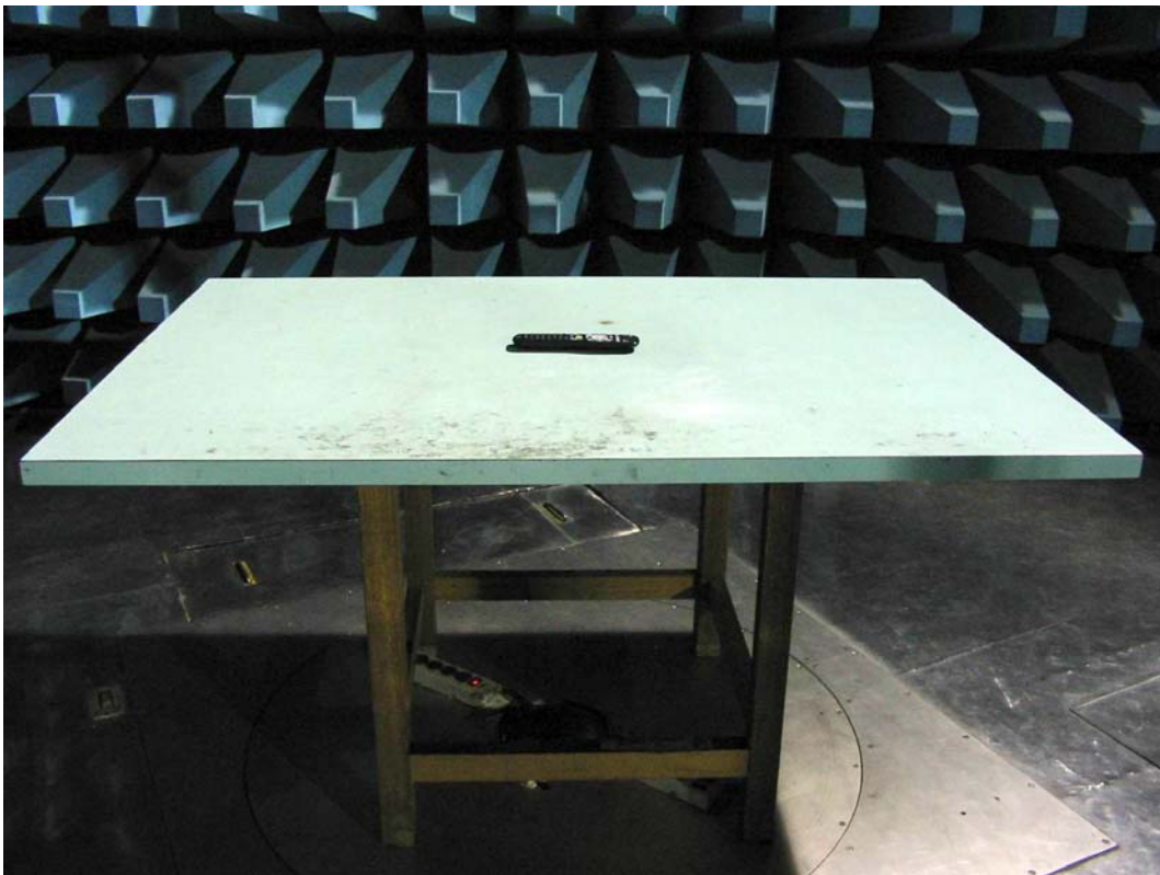
Rear View of the Test Configuration (X-plane)
