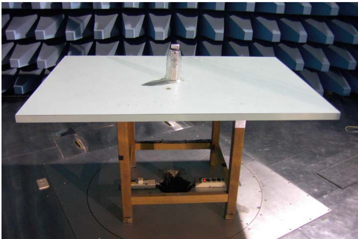
The Test Configuration of Y-plane
