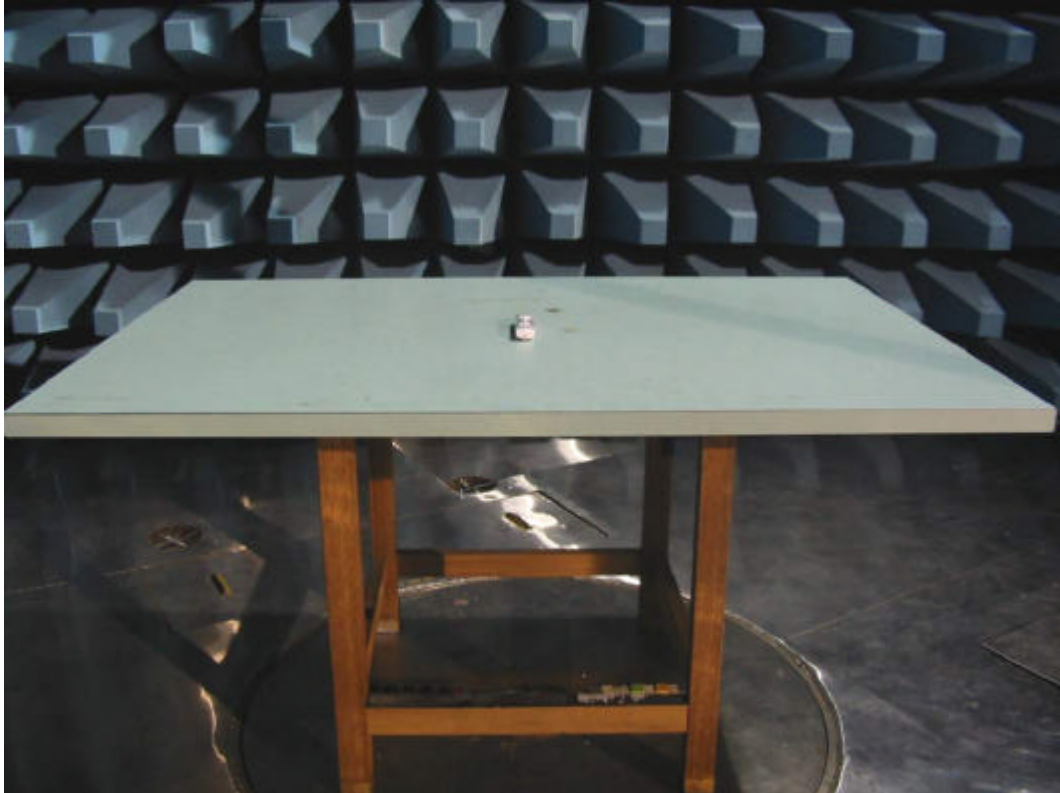
The Test Configuration of Rear view for X-plane
