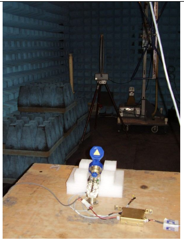
RE test setup in semi-anechoic chamber
