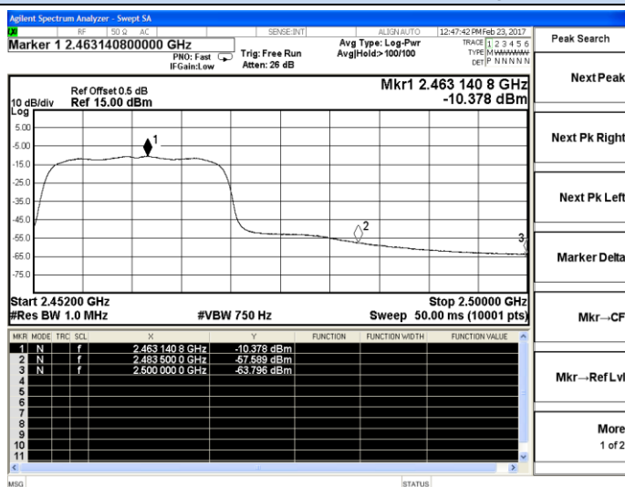
802.11n(HT20)-High channel(Average)
