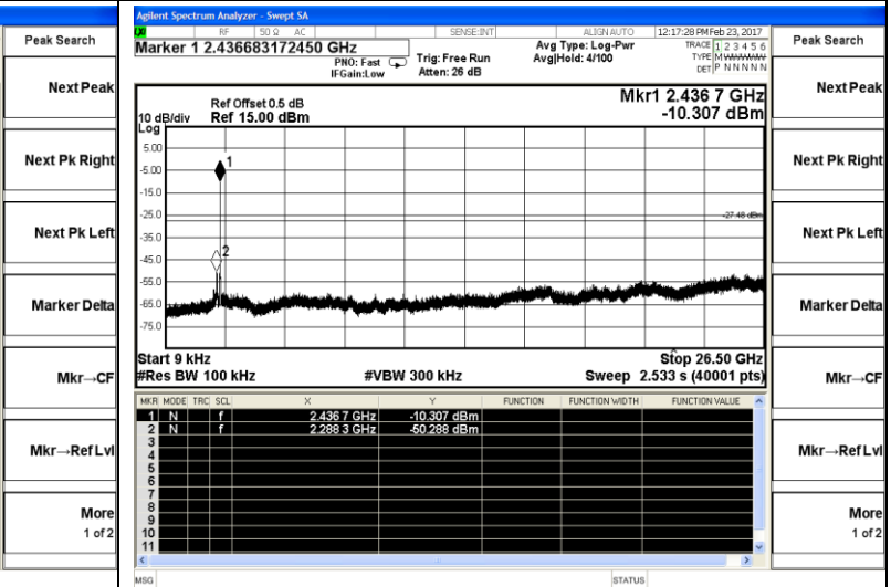
Middle channel
