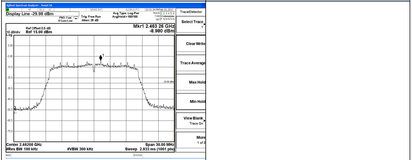
High channel
