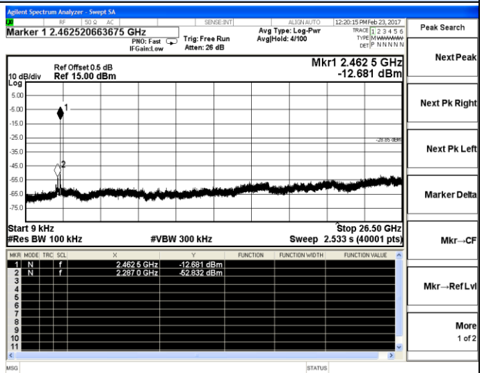
High channel
