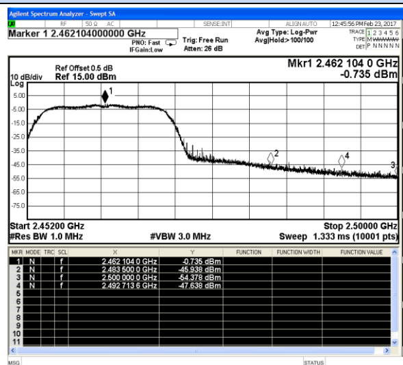
802.11n(HT20)-High channel(Peak)
