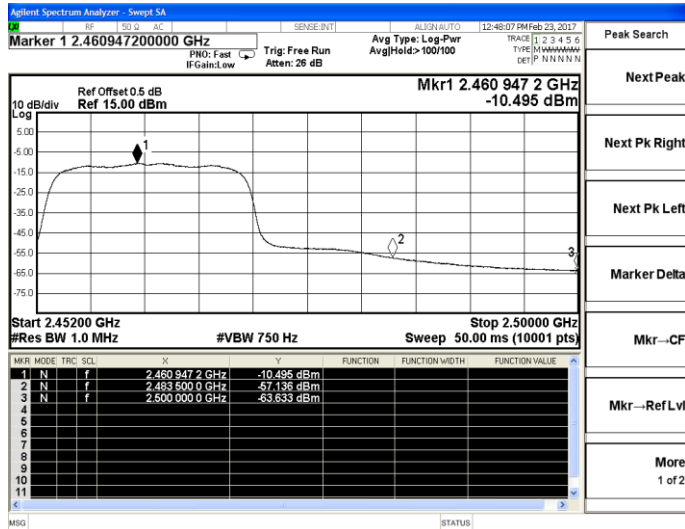
802.11g-High channel(Average)
