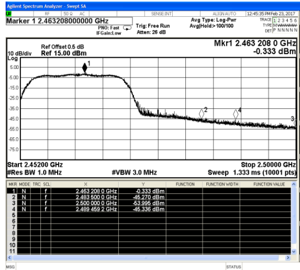
802.11g-High channel(Peak)
