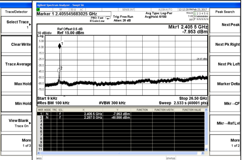
Low channel
