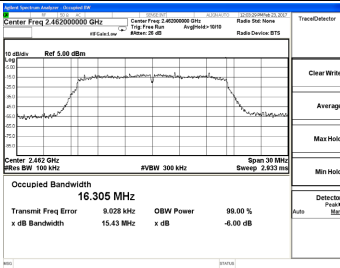
High channel
