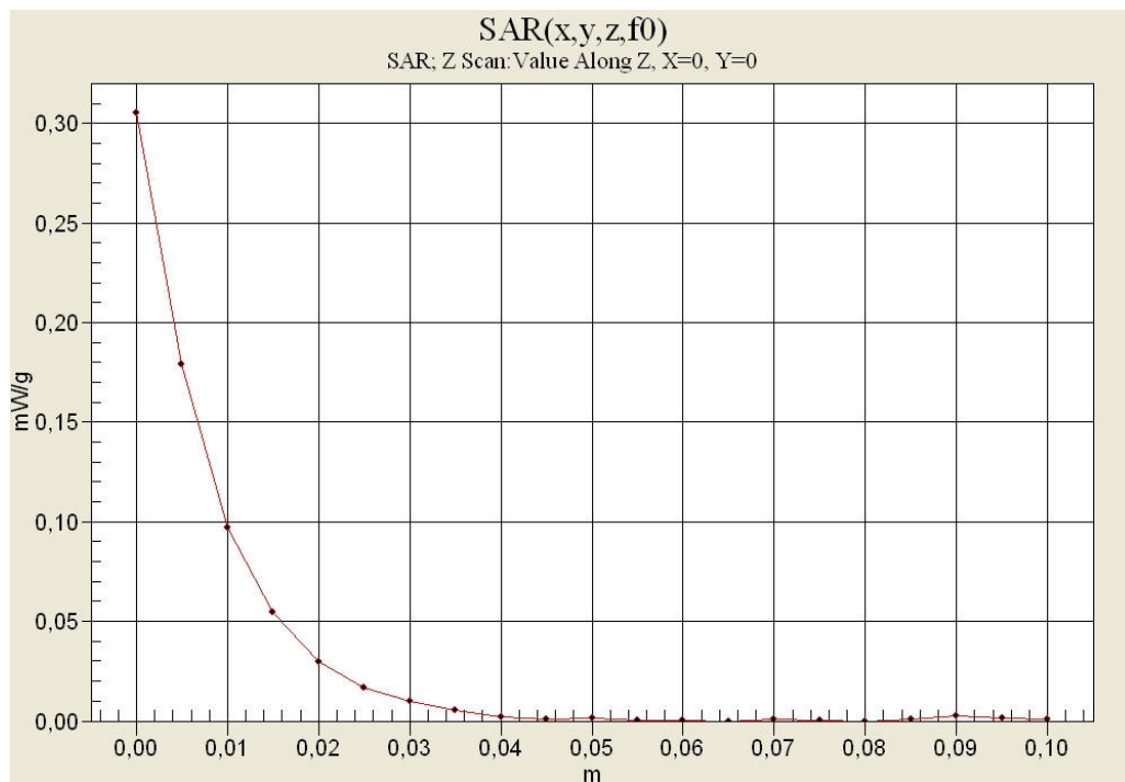
Photo 14: Z-axis scans 2450 MHz body
