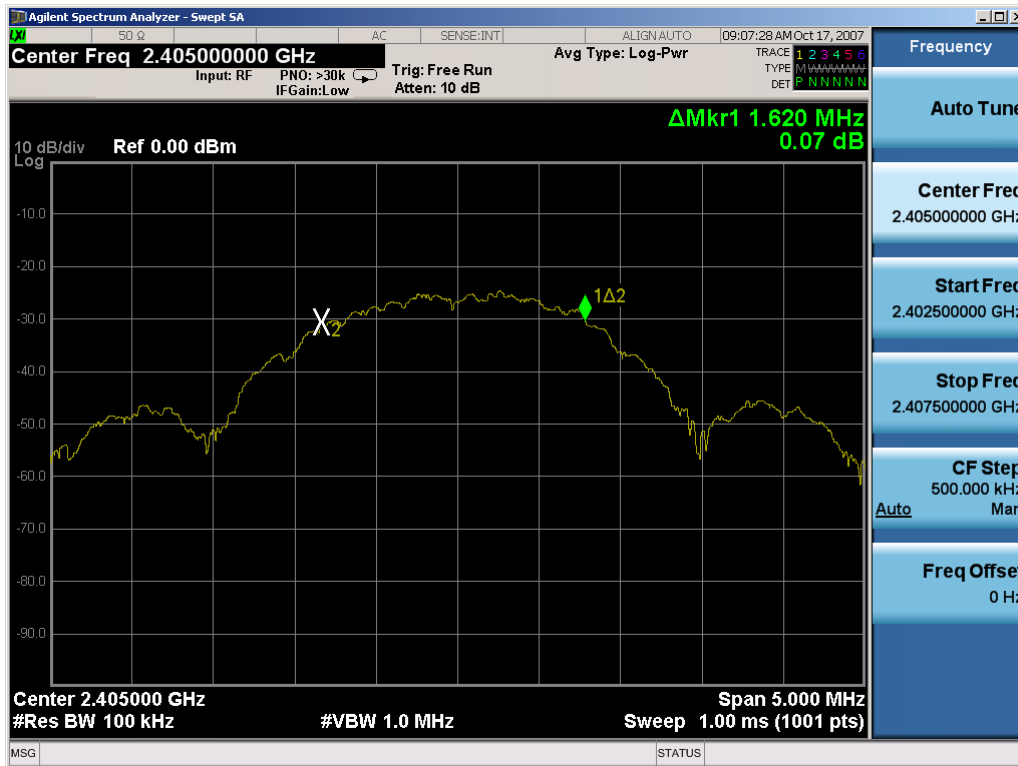
Plot 8-1. Bandwidth Plot Low Channel, 2405 MHz
