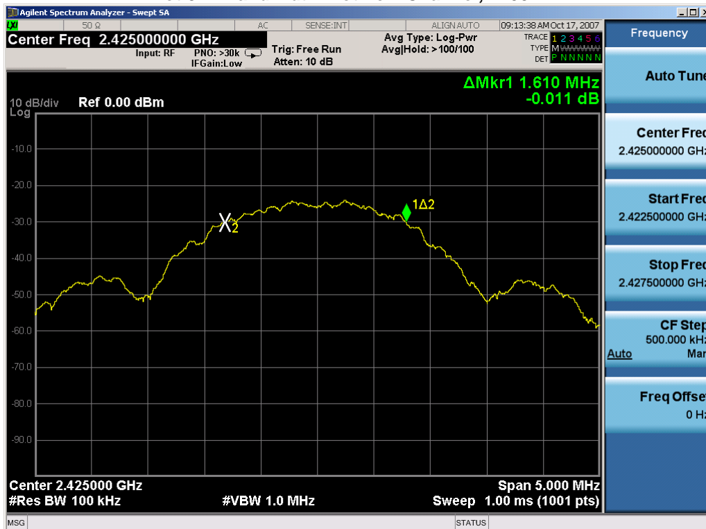
Plot 8-2. Bandwidth Plot Mid Channel, 2425 MHz
