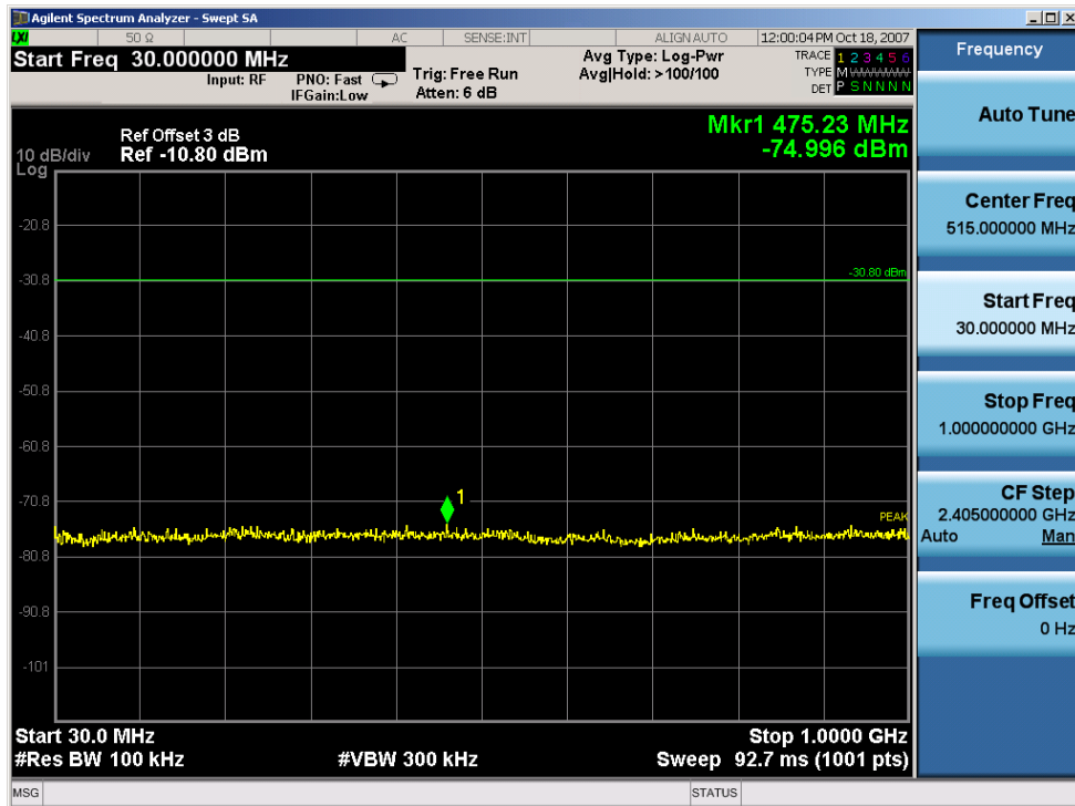
Figure 8-11: 20dBc Spurious Plot, Channel 21
