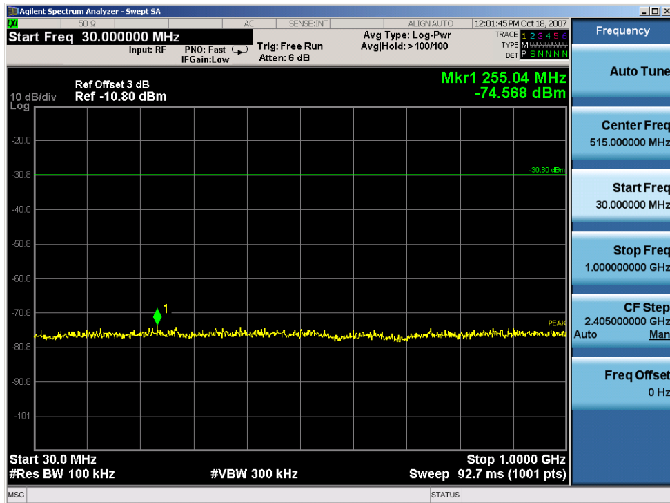
Figure 8-13: 20dBc Spurious Plot, Channel 25
