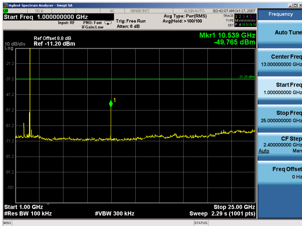
Figure 8-14: 20dBc Spurious Plot, Channel 25
