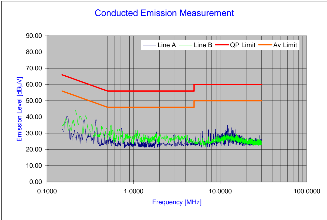
Plot 8-5. Line-Conducted Test Plot
