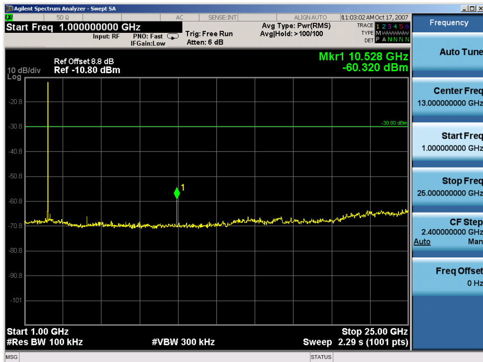
Figure 8-12: 20dBc Spurious Plot, Channel 21
