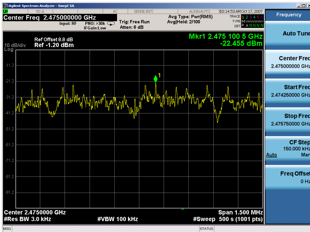
Figure 8-4. PSD Plot, High Channel, 2475 MHz
