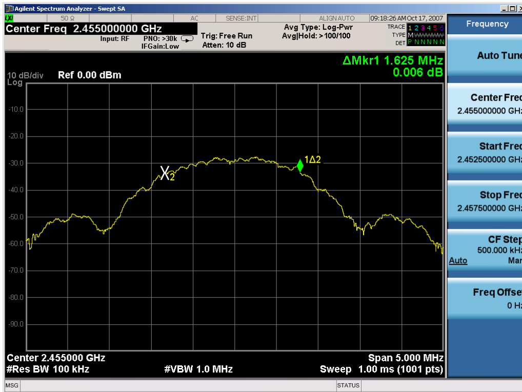
Plot 8-3. Bandwidth Plot Mid Channel, 2455 MHz
