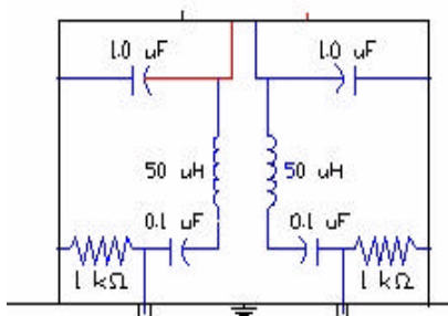
Figure 4. LISN Schematic Diagram
