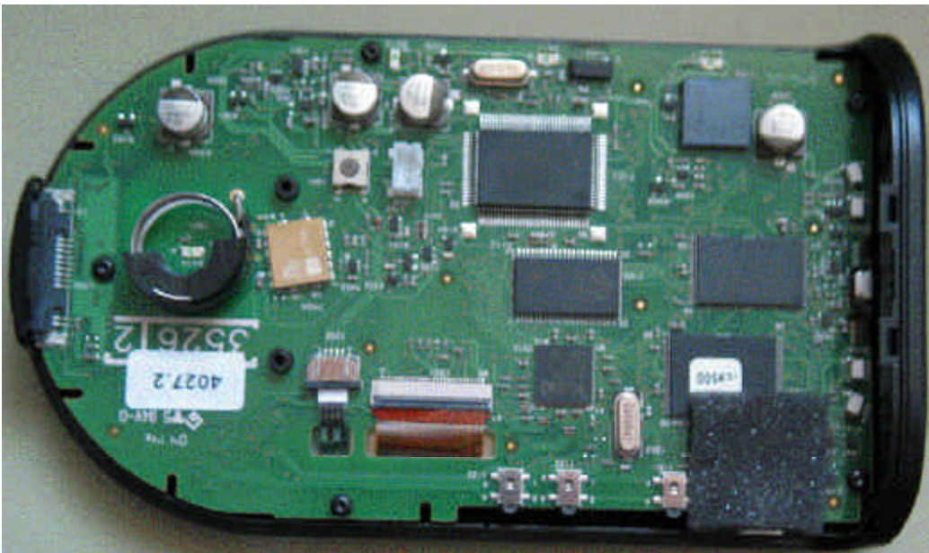
Figure 7 : PWB BOTTOM VIEW
