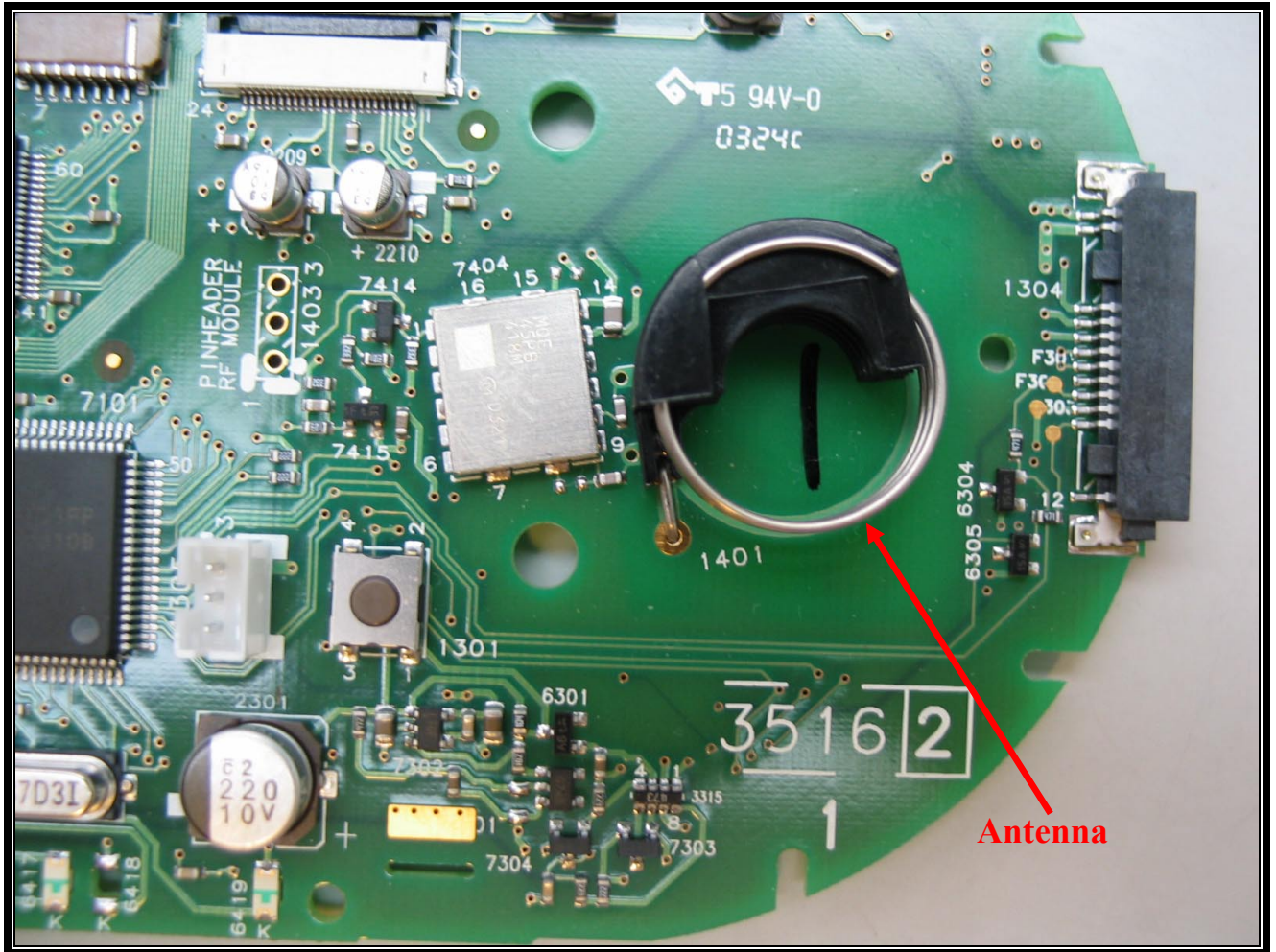
PHOTOGRAPH 21: ANTENNA PART AND MODULE
