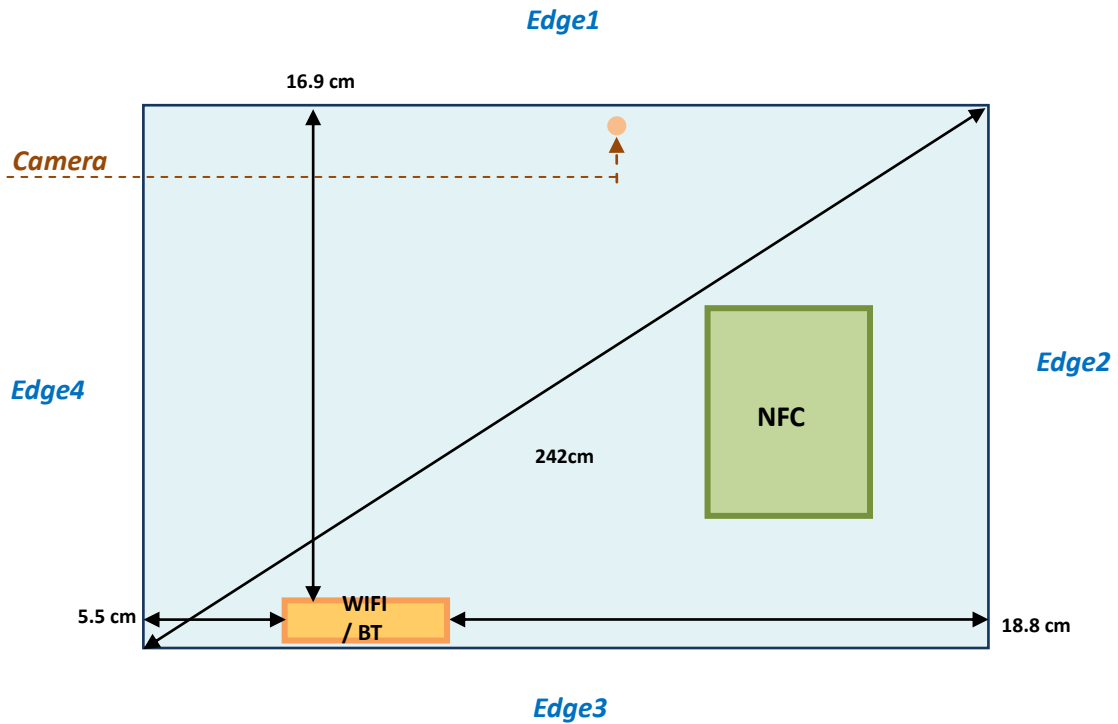
Front View
