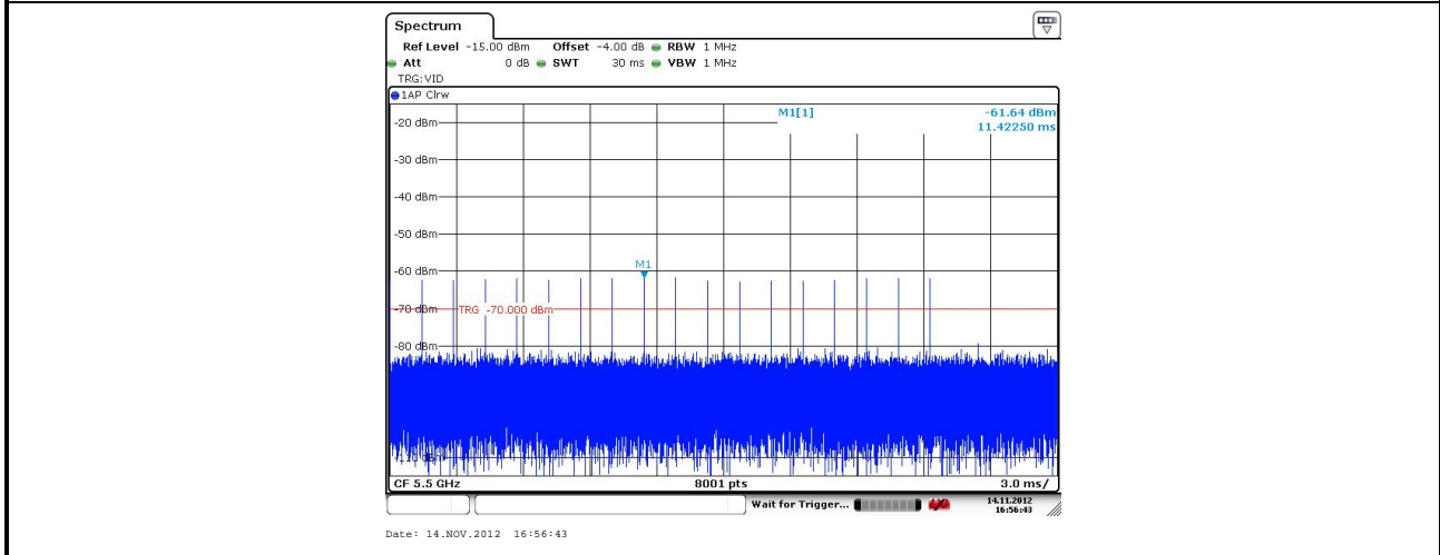
Radar #1 DFS detection threshold level
