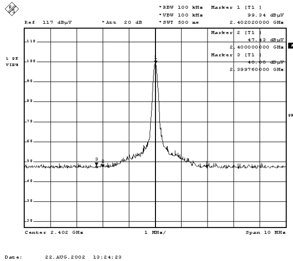
Figure Channel 00: (Vertical)
