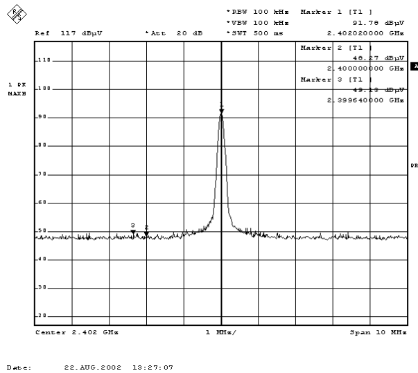
Figure Channel 00: (Vertical)
