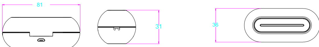
Charging box
