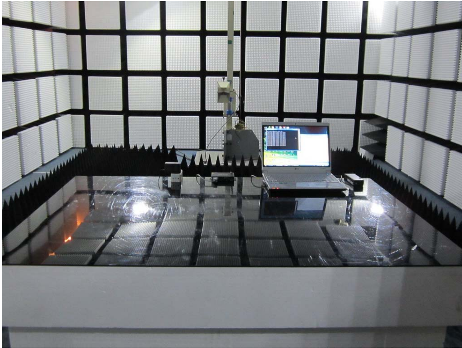
Radiated Emissions above 1 GHz Front View
