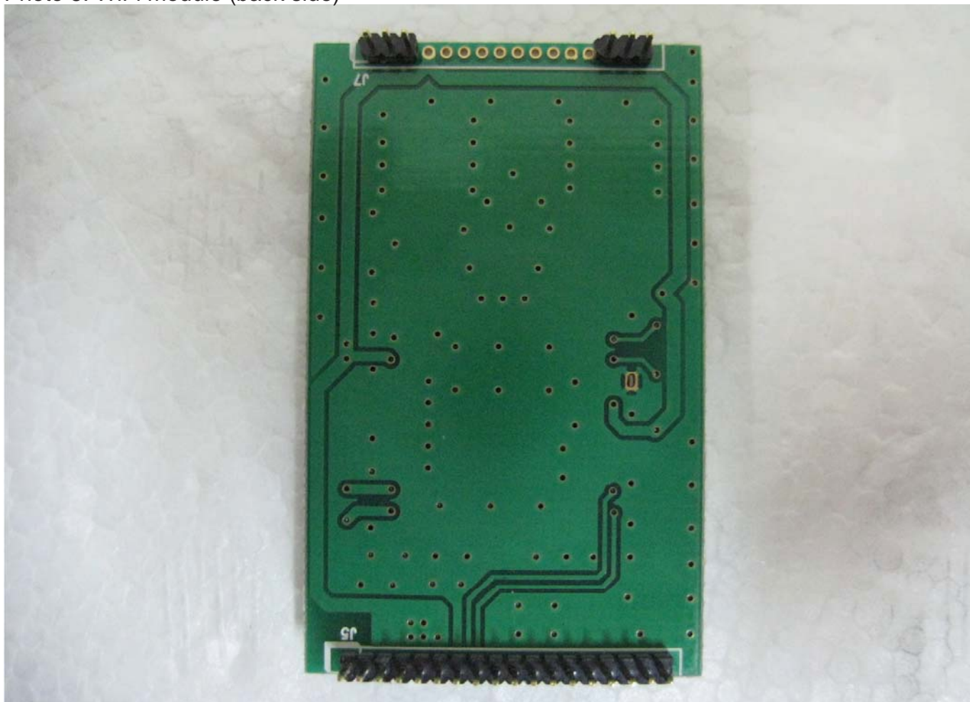
Photo 6: RF board (back side)
