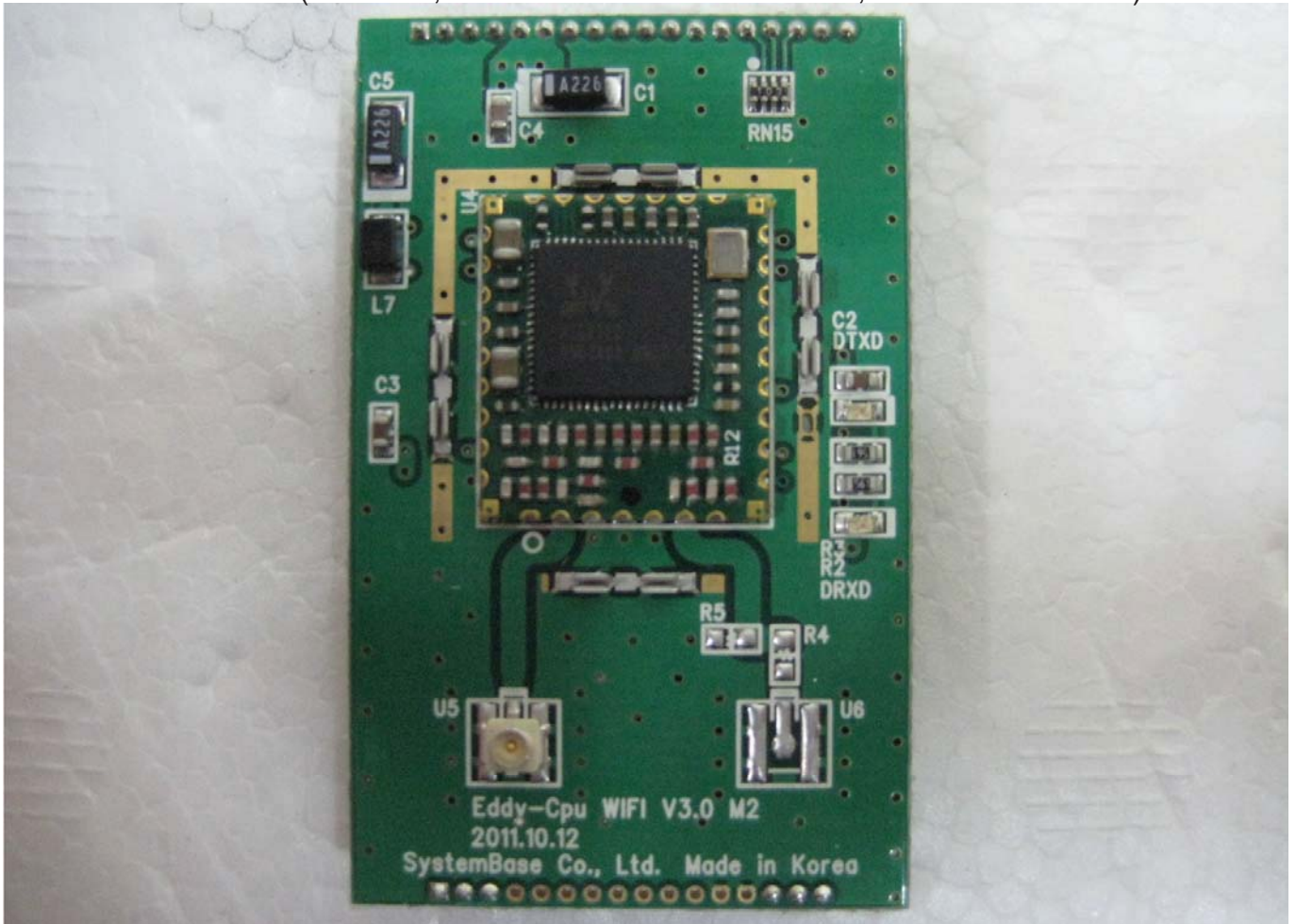
Photo 4: WiFi module (front side, shield removed from RF board, front side RF board)
