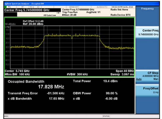
802.11n_HT20 UNII 3 BAND 6dB Bandwidth(CH.149)
