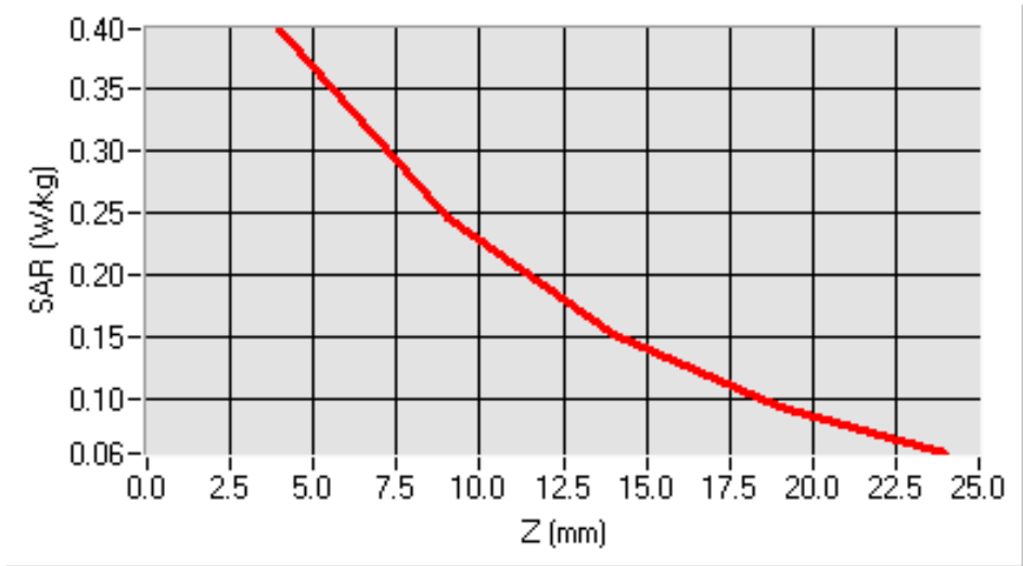
SAR, Z Axis Scan (X = -49, Y = -40)
