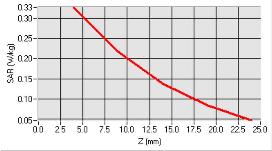
SAR, Z Axis Scan (X = -56, Y = -24)
