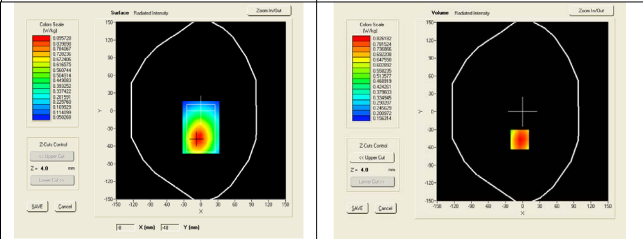
SAR, Z Axis Scan (X = -5, Y = -47)
