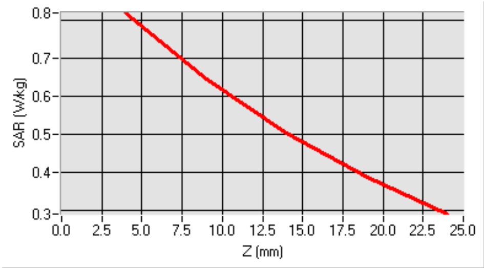
SAR, Z Axis Scan (X = -49, Y = -32)
