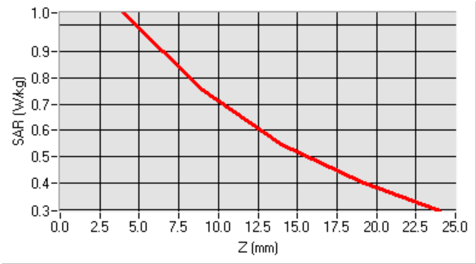
SAR, Z Axis Scan (X = 2, Y = -46)
