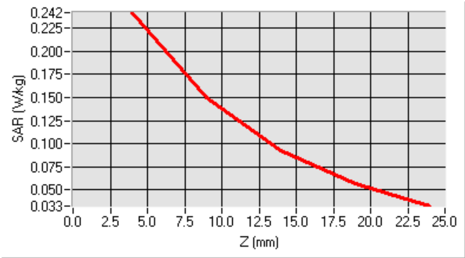
SAR, Z Axis Scan (X = -8, Y = -57)
