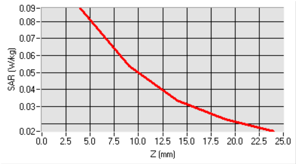
SAR, Z Axis Scan (X = -47, Y = -40)
