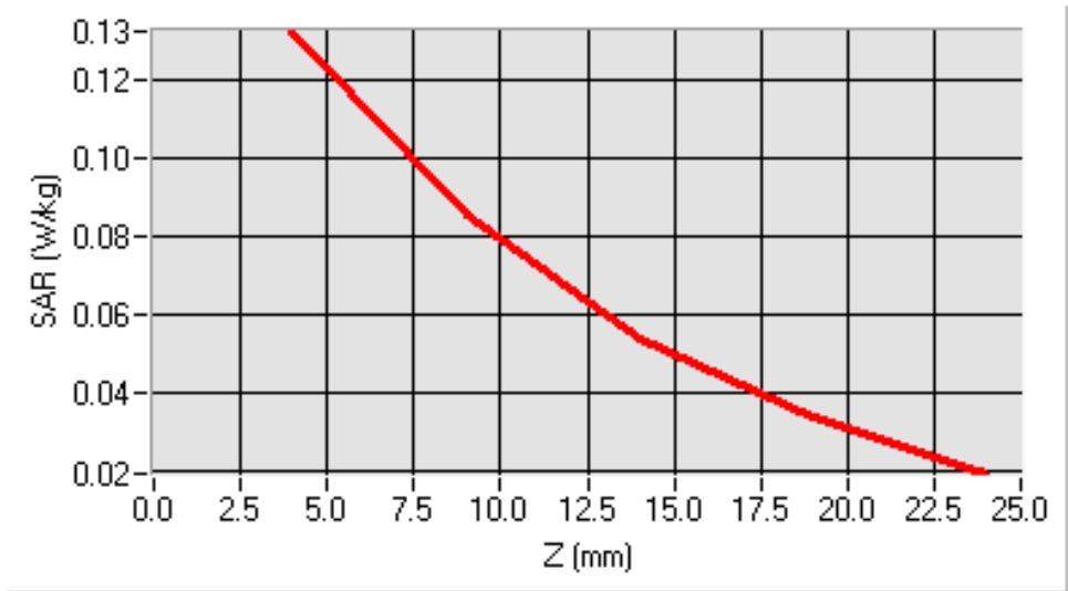
SAR, Z Axis Scan (X = -54, Y = -22)
