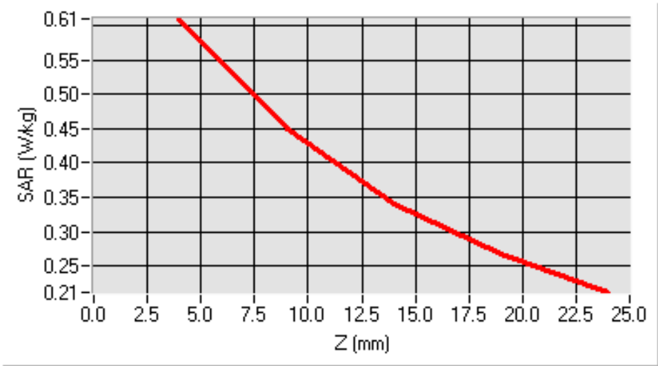
SAR, Z Axis Scan (X = -33, Y = -18)
