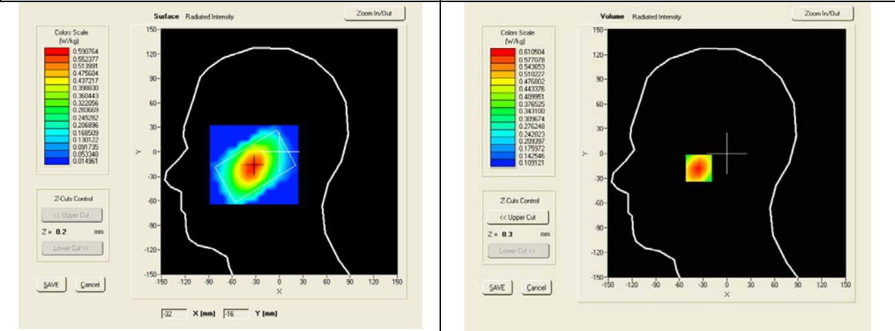
SAR, Z Axis Scan (X = -33, Y = -18)
