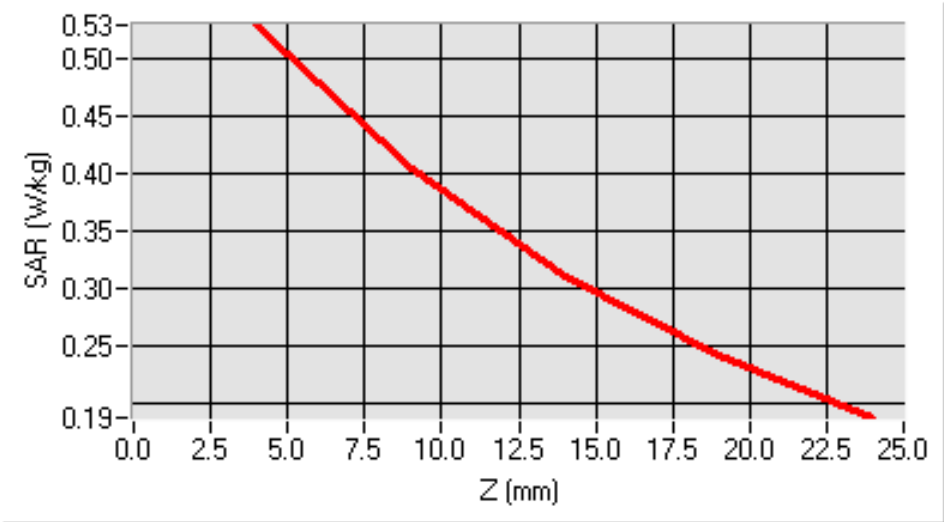
SAR, Z Axis Scan (X = -34, Y = -18)
