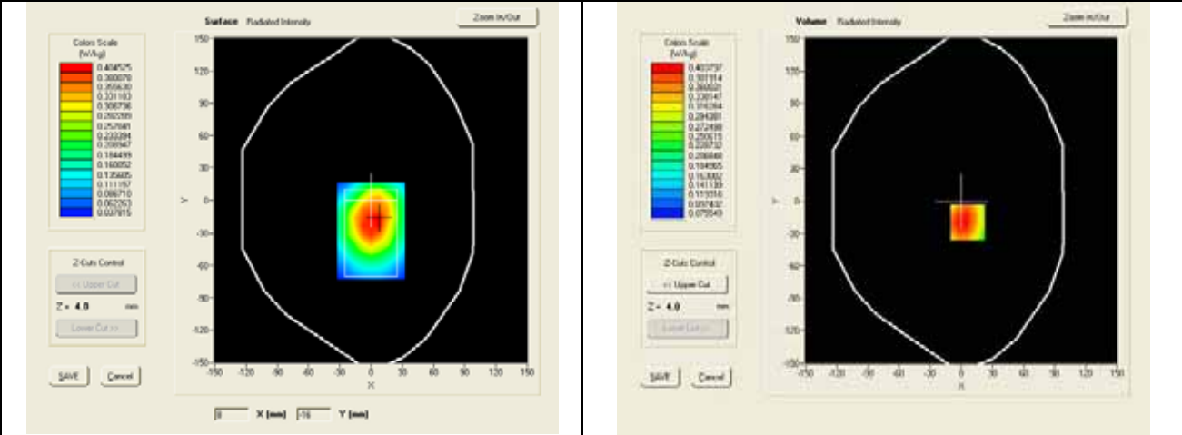
SAR, Z Axis Scan (X = 6, Y = -20)
