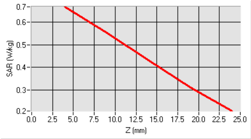
SAR, Z Axis Scan (X = -23, Y = -2)
