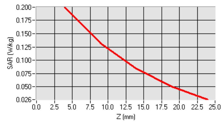
SAR, Z Axis Scan (X = 10, Y = -13)
