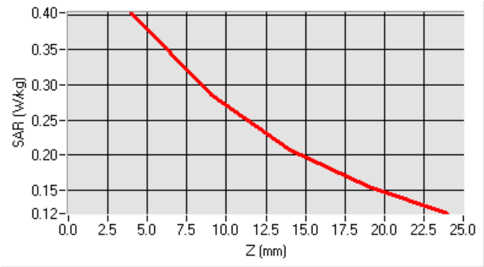
SAR, Z Axis Scan (X = 6, Y = -20)
