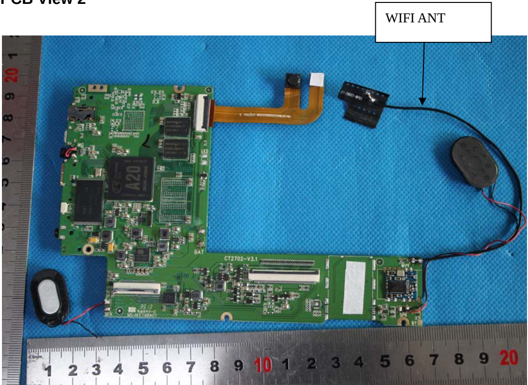
EUT – PCB View 2
