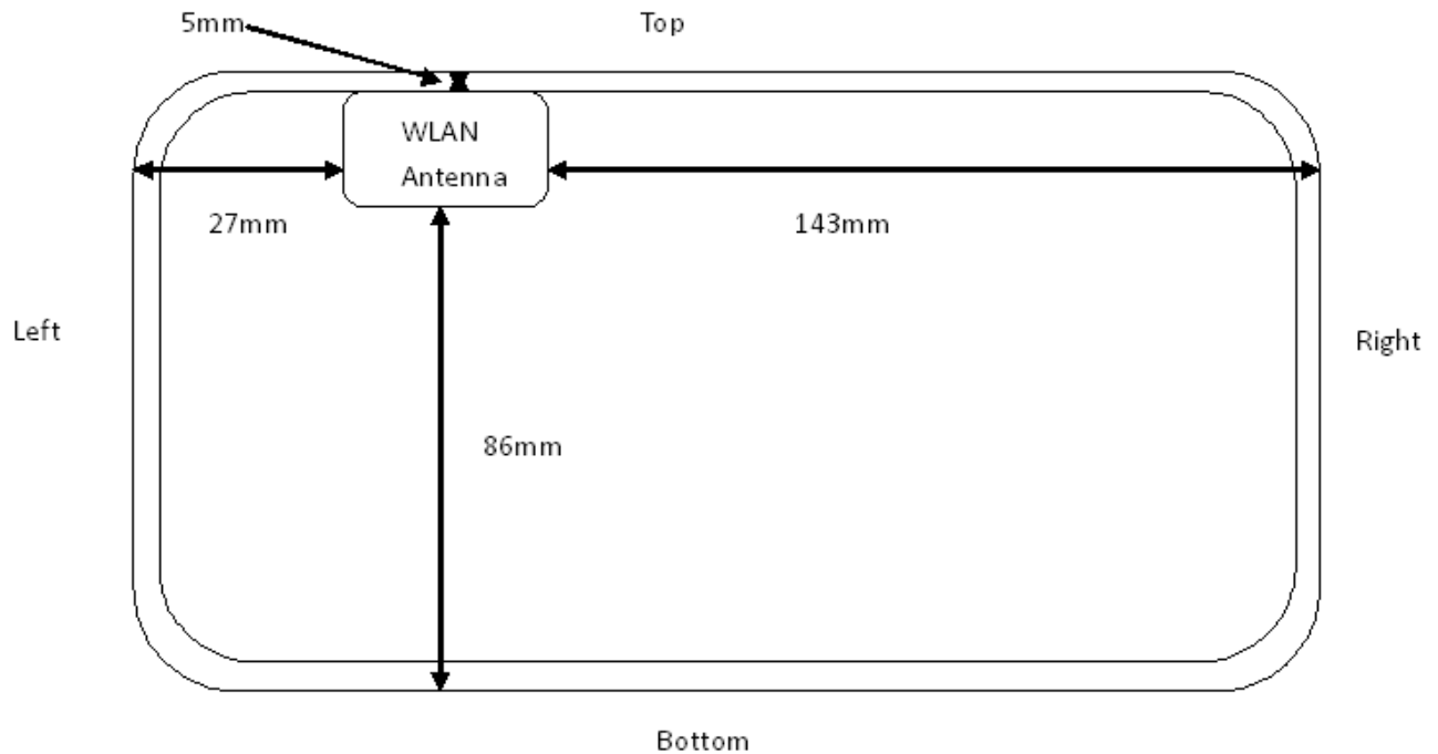
Posiotions of Antenna
