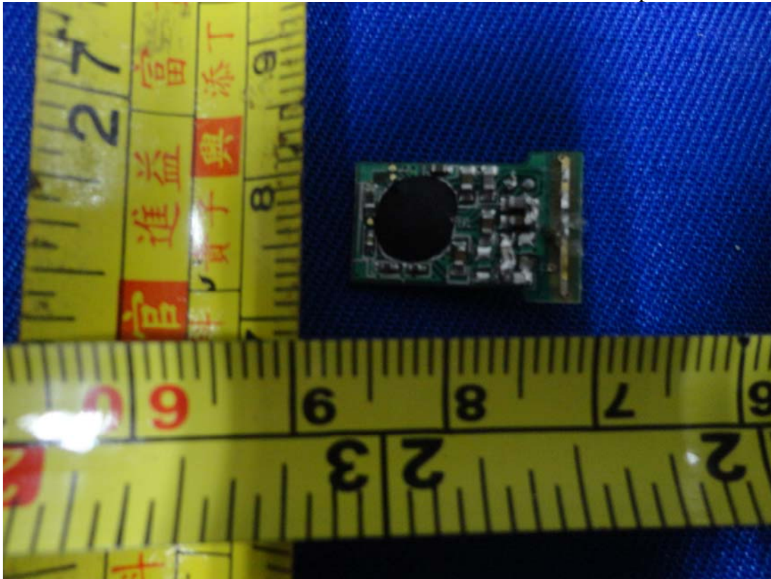
Figure 1 Component Side of the PCB
