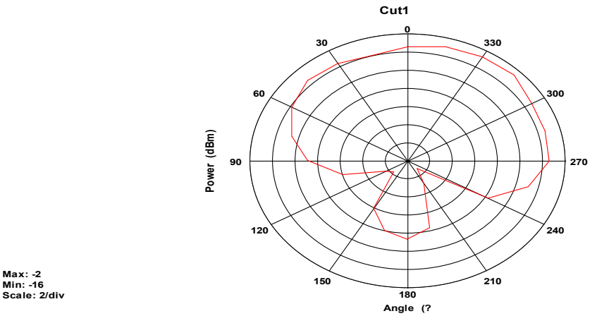
2440M TRP 1
