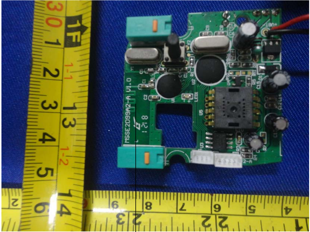
Figure 3 Component Side of the PCB
